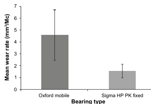
Figure 12 Reduced wear in DePuy partial knee, compared with conforming Oxford knee.
