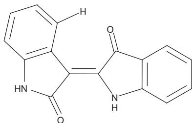
Figure 1 Chemical structure of indirubin.
