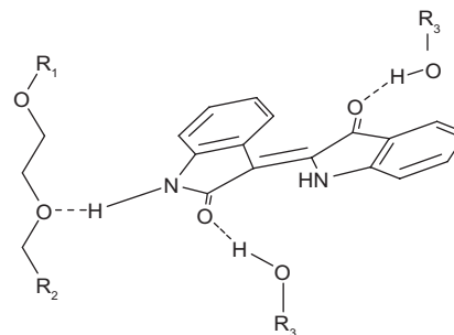
Figure 4D Schematic diagram of hydrogen bonds between indirubin and PEG 4000.
