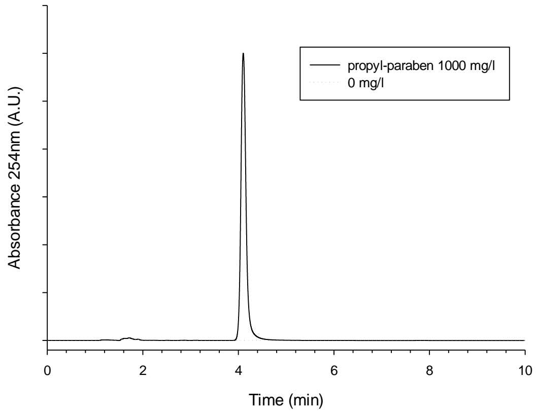
Figure S2. Chromatogram of a propyl-paraben solution 1 mg/ml and pure solvent
