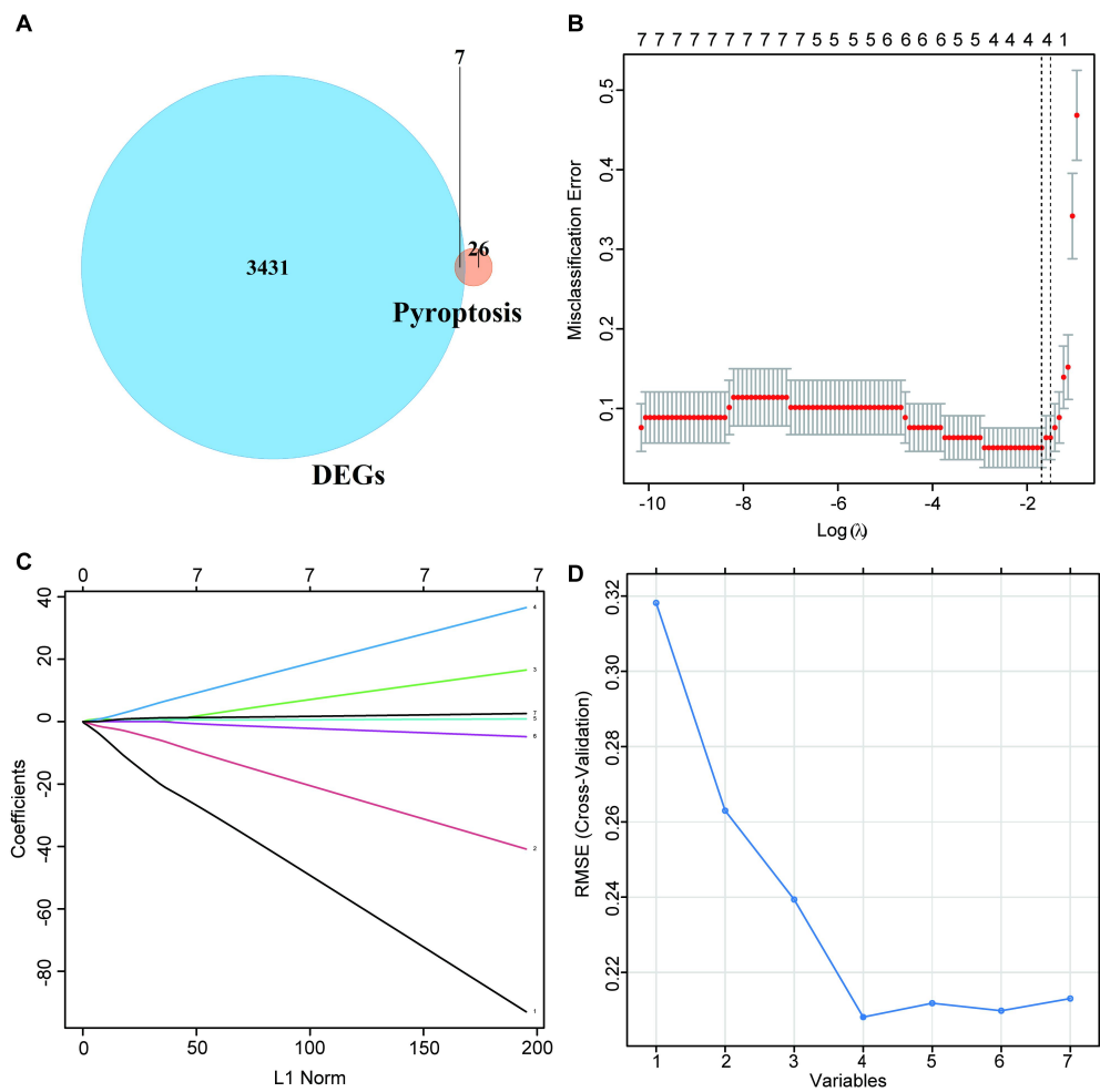
Figure S1. Identified differentially expressed pyroptosis-related genes (DPRGs). (A) Venn diagram analysis showed that the overlap of differentially expressed genes and 33 pyroptosis-related genes led to seven DPRGs being identified. (B) Cross-validation for tuning parameter selection in the LASSO (least absolute shrinkage and selection operator) model. The cross-validation error was minimal when five genes were selected. (C) LASSO coefficient profiles of the seven DPRGs. (D) Bouts of cross-validation error was minimal when four DPRGs were selected by SVM-RFE (support vector machine recursive feature elimination) algorithms.
