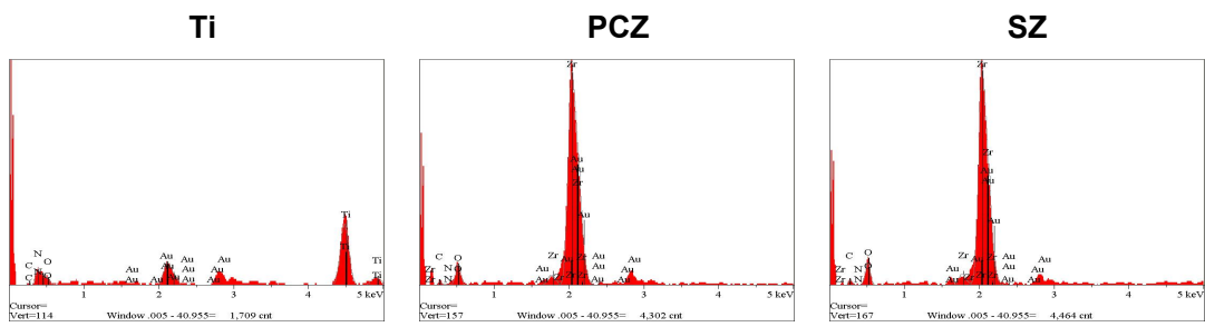
Supplementary figure 1: The EDS energy spectrum of Ti, PCZ, and SZ samples.
