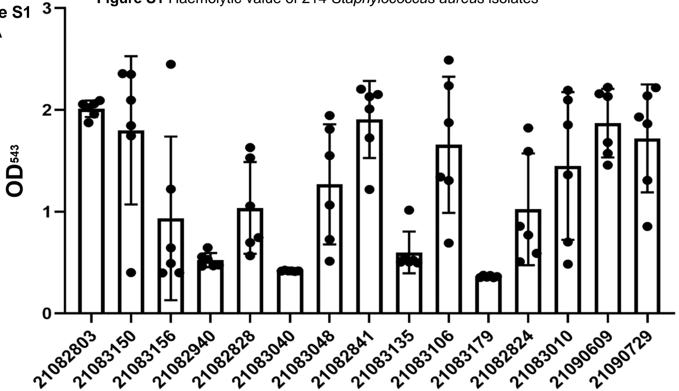
Figure S1 Haemolytic value of 214 Staphylococcus aureus isolates
