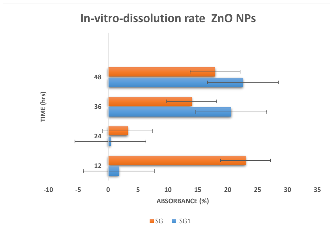
Figure S1: In-vitro bioavailability study. (A) Scheme. (B) Graph.
