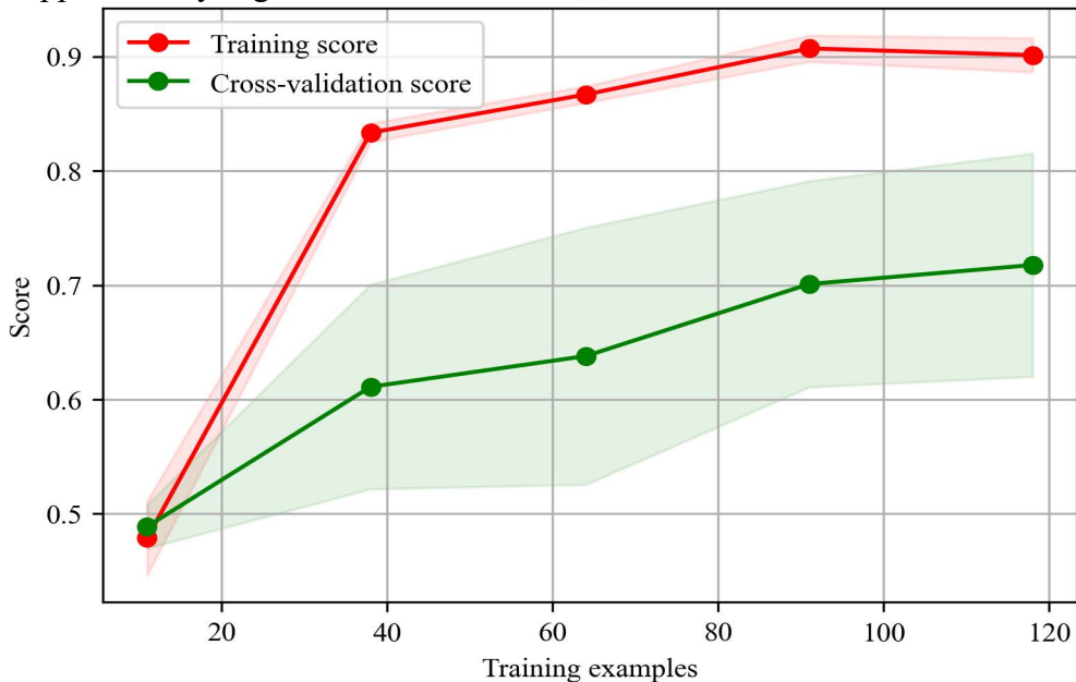
Supplementary Figure 1: the learning curve of the final prediction model
