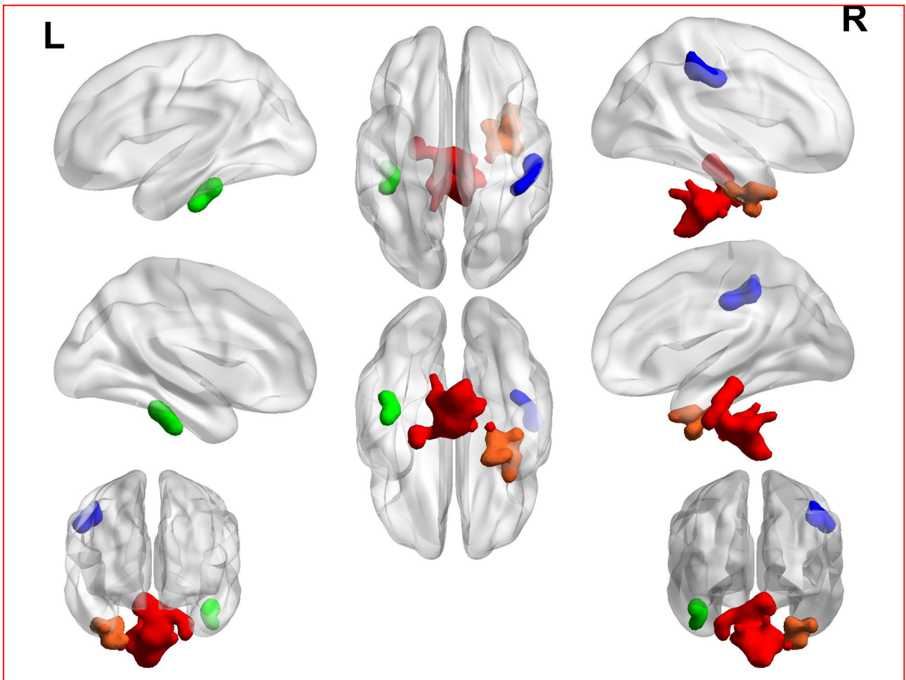
Fig S1 This results were similar to Fig5A between 20 male pre-CAPA OSA patients and 20 HC groups in the typical frequency band (0.01-0.08 Hz), indicated that the stability of the results was independent of gender.
