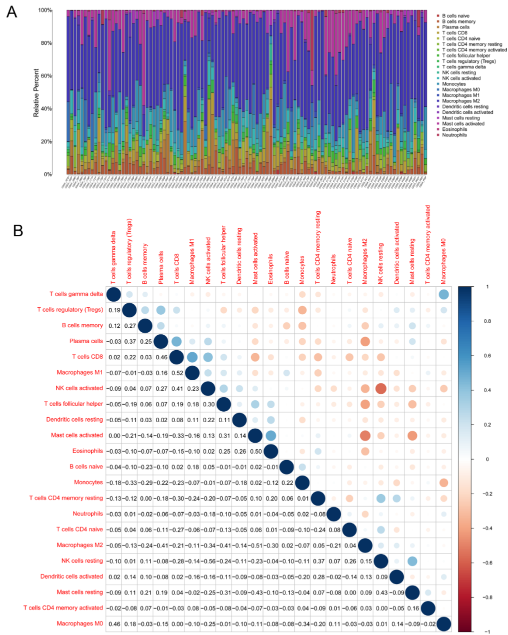
Figure S1: TICs profiles of validation data set.
