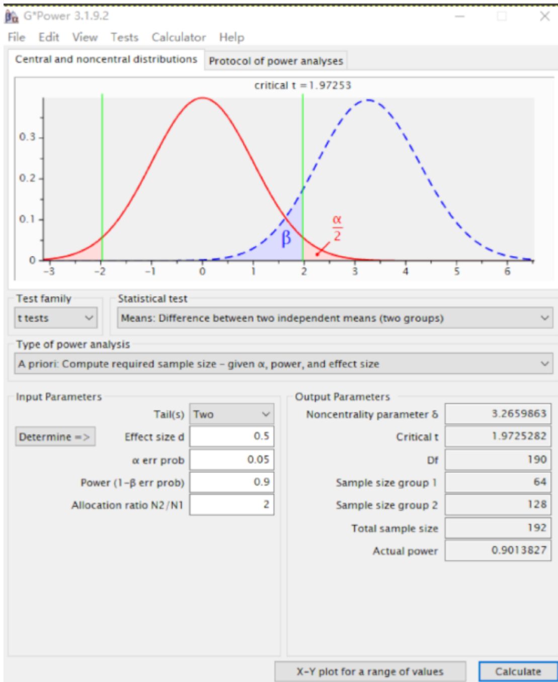
Supplementary Figure 1 Gpower was used to calculate the sample size.
