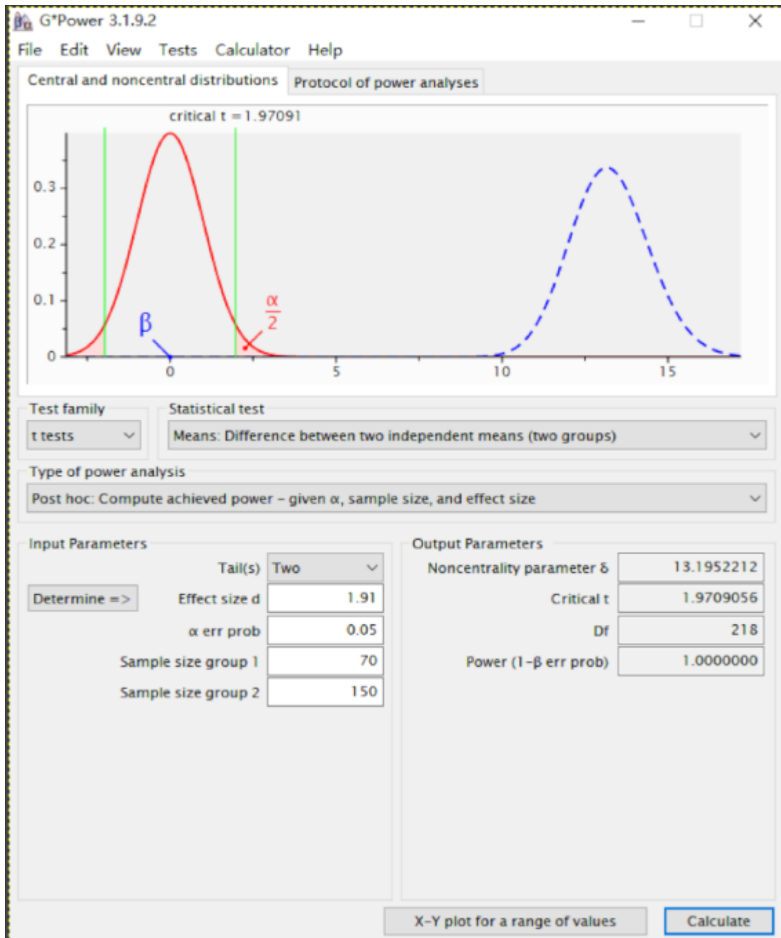
Supplementary Figure 2 Gpower was used to calculate the statistical effect of lncRNA HEIH expression difference between the control group and NSCLC group.
