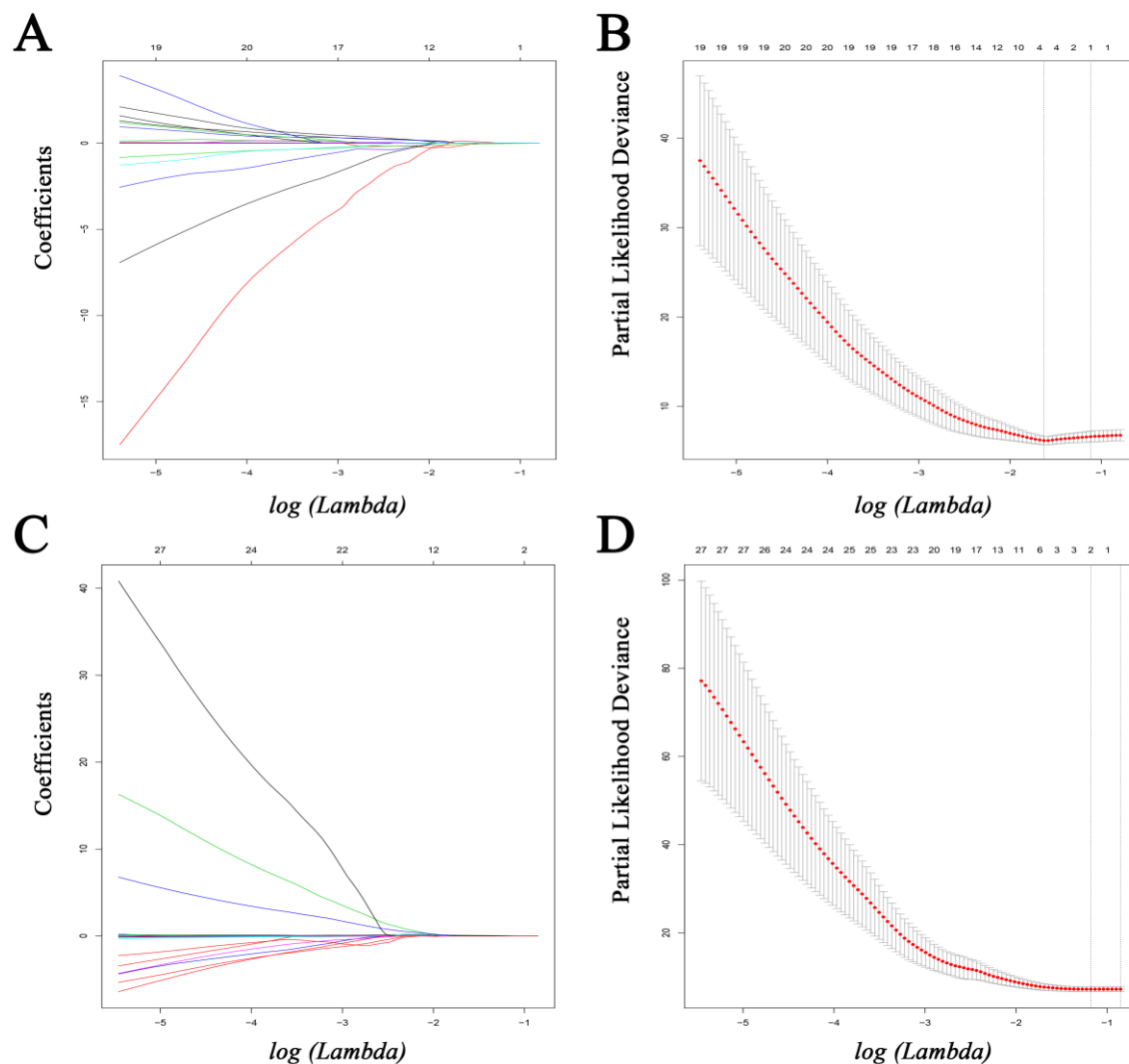
Supplementary Figure 1 Feature selection using the least absolute shrinkage and selection operator (LASSO) Cox regression model. A. LASSO coefficient profiles of variables against the \log(\text{Lambda}) sequence for OS. B. The tuning parameter ( \text{Lambda} ) selection in the LASSO model used 10-fold cross-validation via minimum criteria for OS. C. LASSO coefficient profiles of 48 variables against the \log(\text{Lambda}) sequence for OS. D. The tuning parameter ( \text{Lambda} ) selection in the LASSO model used 10-fold cross-validation via minimum criteria for OS. OS, overall survival; PFS, progression-free survival.
