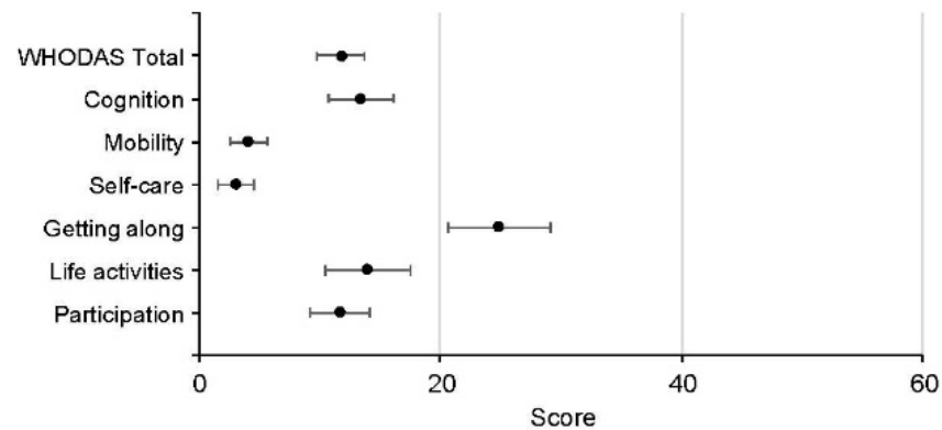
(C) SR LOCF=No, Achieved goal=Yes
