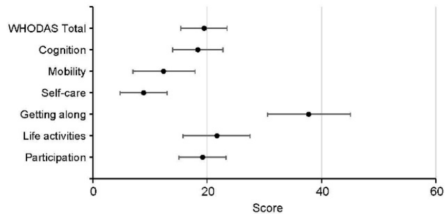
(C) SR LOCF=No, Achieved goal=Yes
