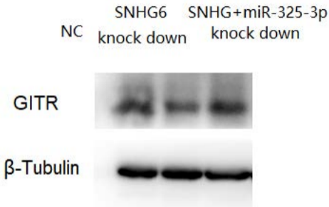
Figure S1: GITR expression detected by western blot in MKN45 cell line
