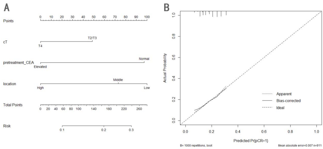
Figure S1. Nomogram and calibration curves for pCR
