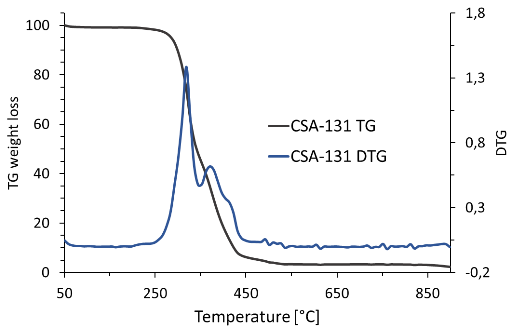
Supplementary Figure 1. TD and DTG of ceragenin CSA-131
