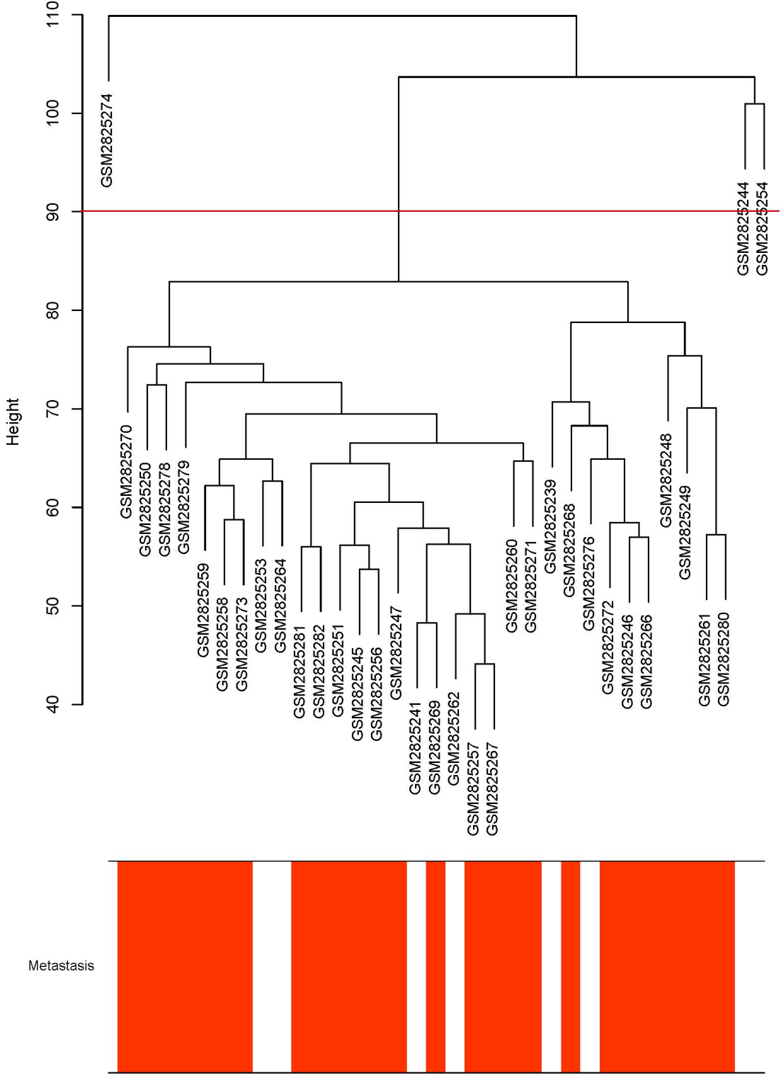
Sample dendrogram and trait heatmap
