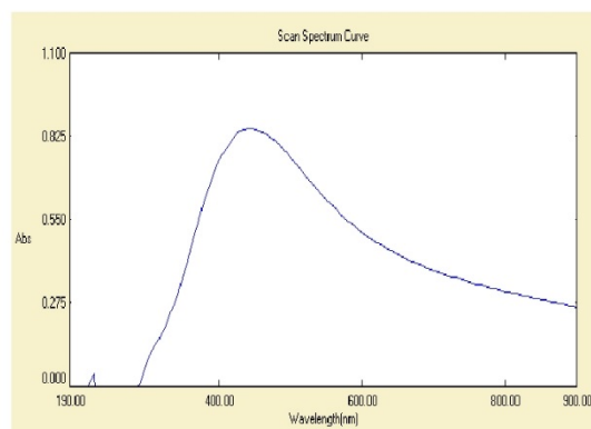
Figure 1: UV-Visible spectrum of SeNPs synthesized by using compound (2b) at room temperature.
