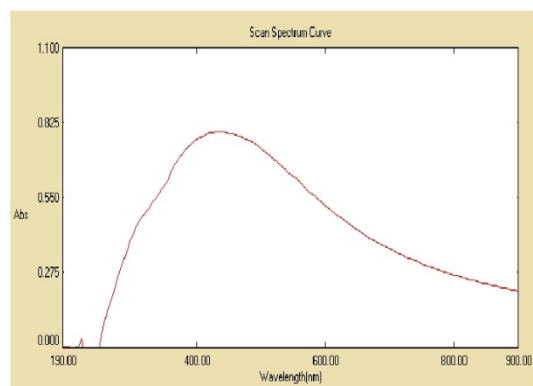
Figure 2: UV-Visible spectrum of SeNPs synthesized by using compound (2c) at room temperature.
