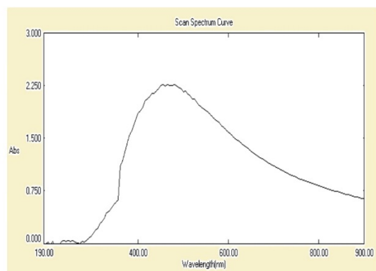
Figure 4: UV-Visible spectrum of SeNPs synthesized by using compound (2g) at room temperature.
