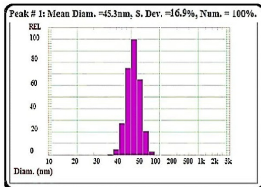
Figure 9: DLS pattern of particle size distribution of the SeNPs synthesized by using compound (2g) at room temperature.
