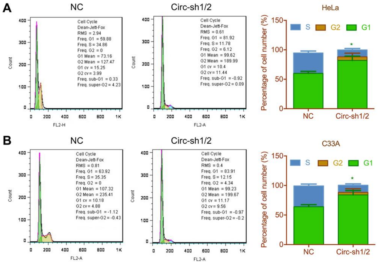
Figure S1. Knockdown of circ_103973 accelerated cell cycle arrest of HeLa and C33A cells. HeLa and C33A cells were transfected with NC and circ_103973 siRNAs, respectively. Cell cycle distribution was examined by Flow cytometry in HeLa (A) and C33A (B) cells. *P < 0.05.
