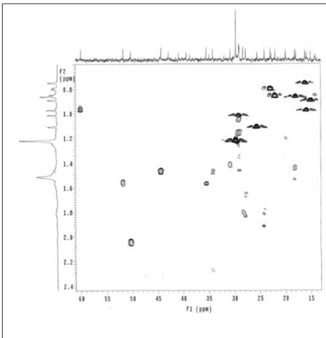
Supplementary Figure 7 HSQC spectrum of 7\beta,19\alpha dihydroxy-urs-12-ene (6)
