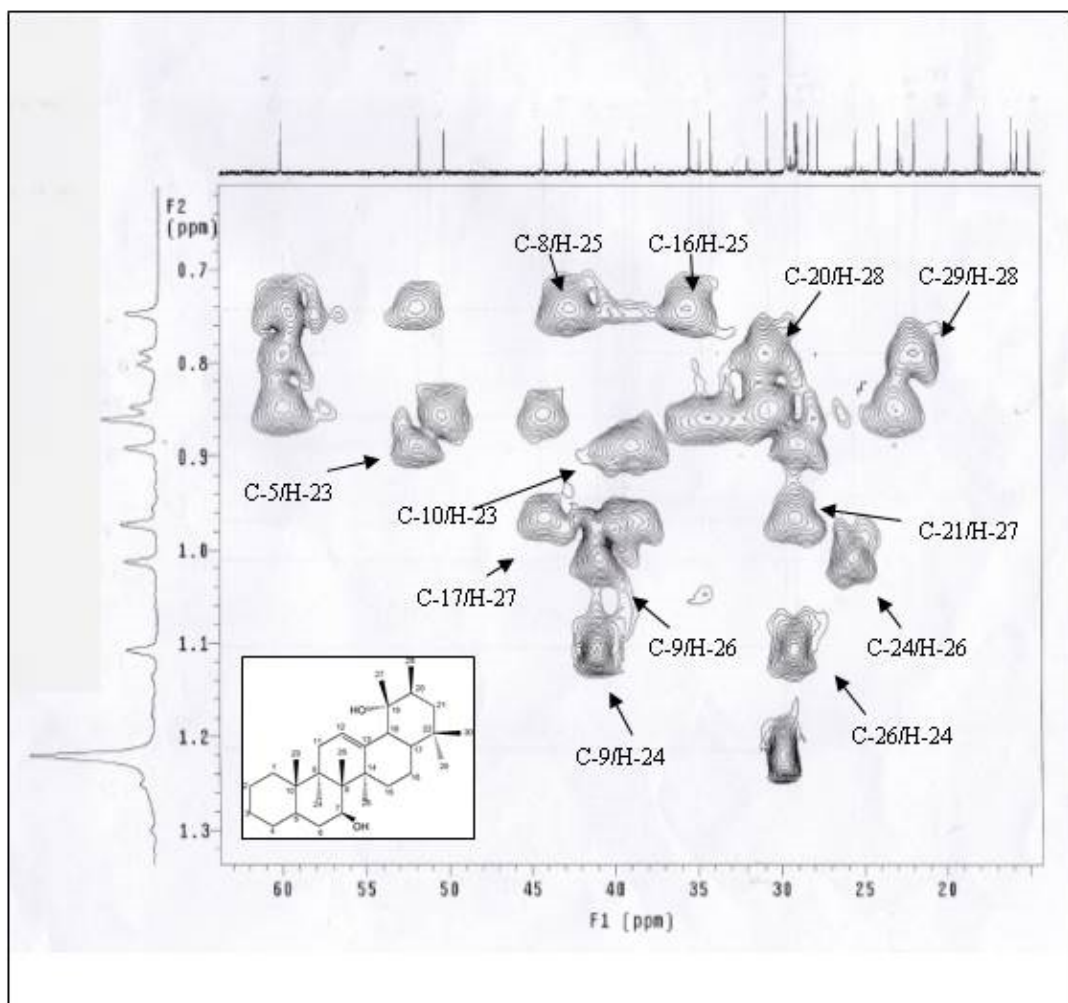
Supplementary Figure 8 HMBC spectrum of 7β,19α dihydroxy-urs-12-ene (6)
