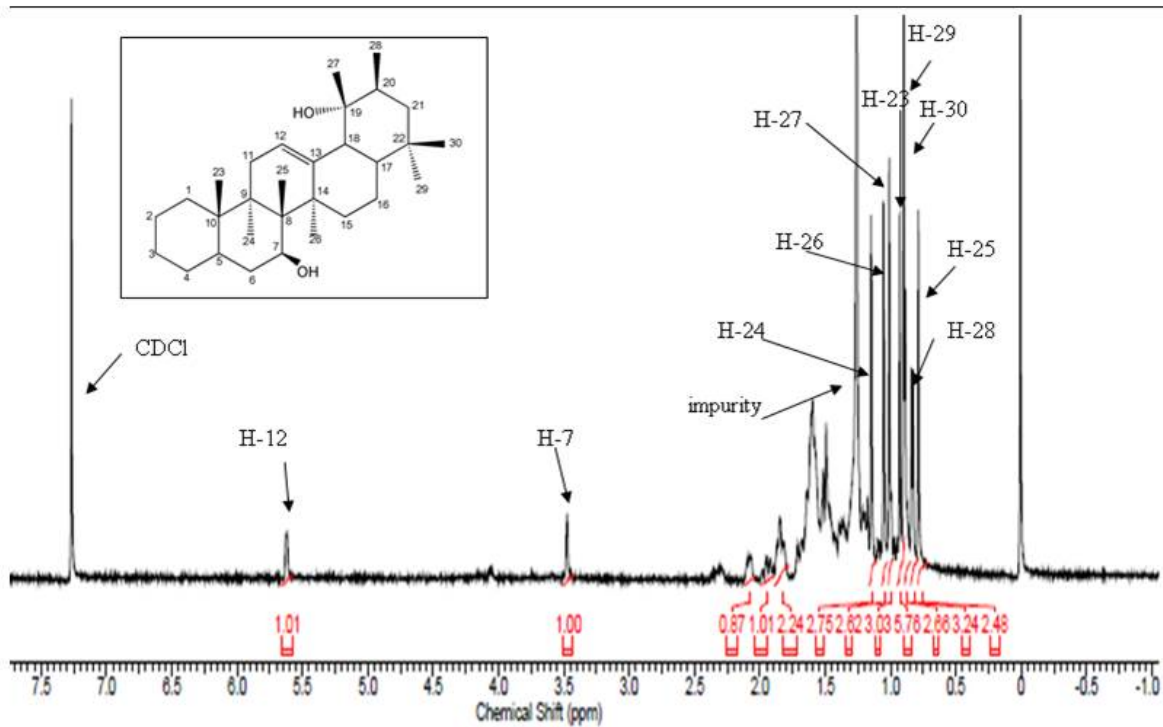
Supplementary Figure 3 1 H NMR spectrum of 7β,19α dihydroxy-urs-12-ene (6)
