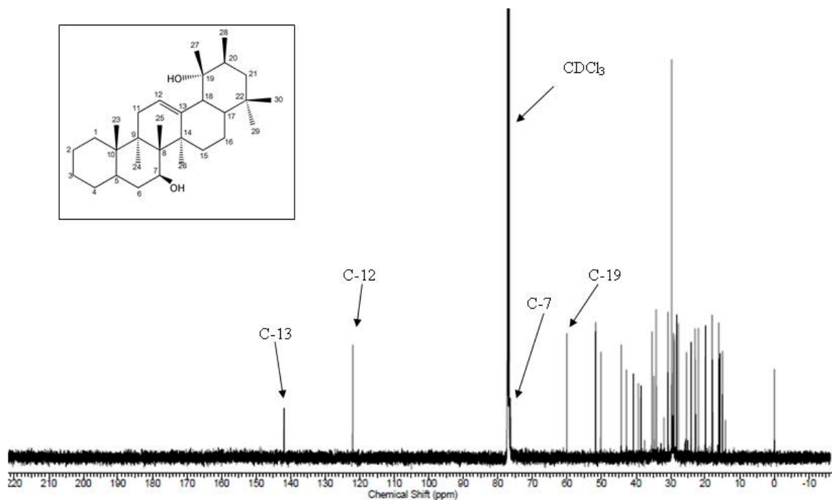
Supplementary Figure 4 13 C NMR spectrum of 7β,19α dihydroxy-urs-12-ene (6)
