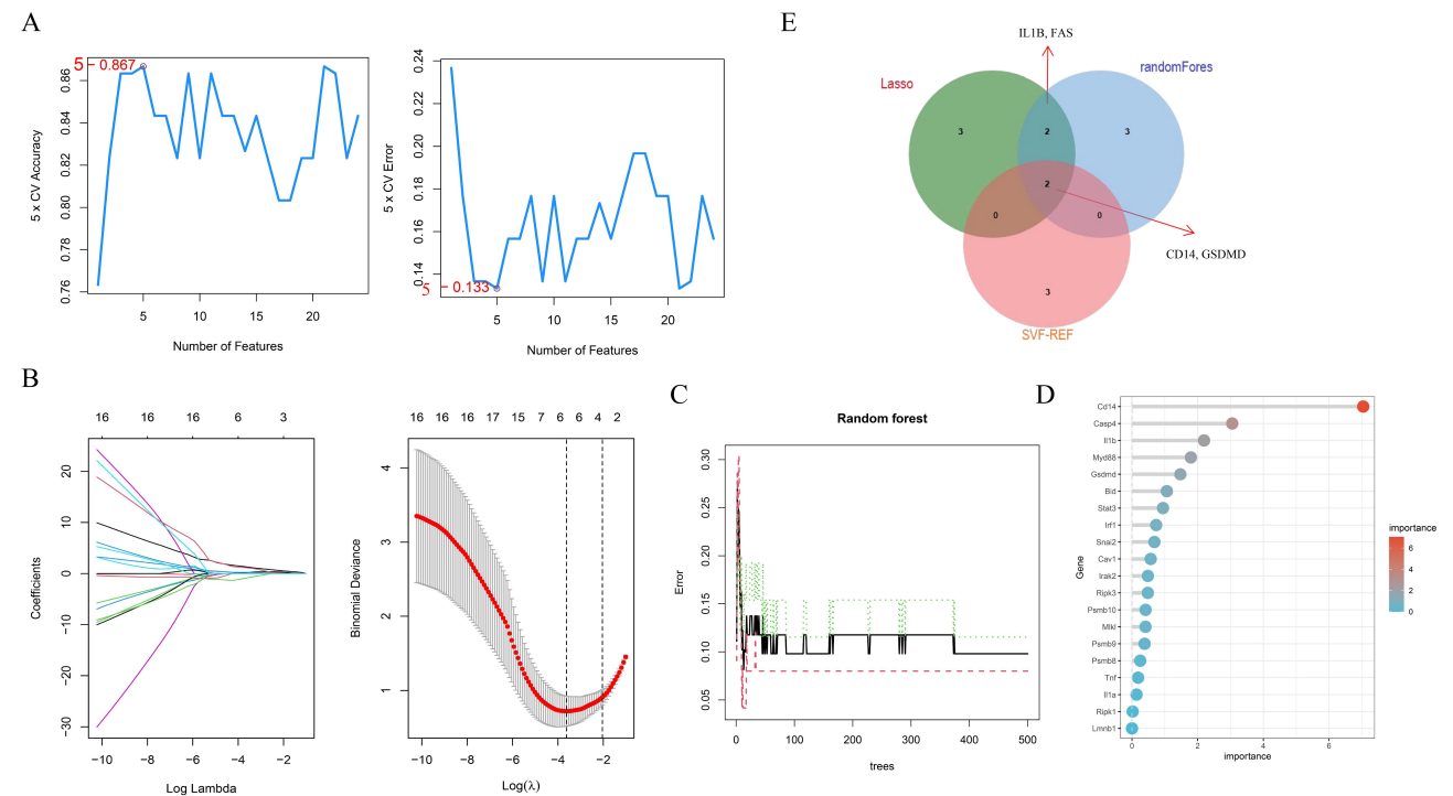
Figure 3 Signature genes selection. (A) The accuracy curve and error rate curve for 5-fold cross-validation based on SVM-RFE algorithm. (B) Lasso regression plot and 10-fold cross-validation plot. (C) RF error rate versus the number of classification trees. (D) The top 20 relatively significant genes based on RF algorithm. (E) Three algorithmic Venn diagram screening signature genes.
