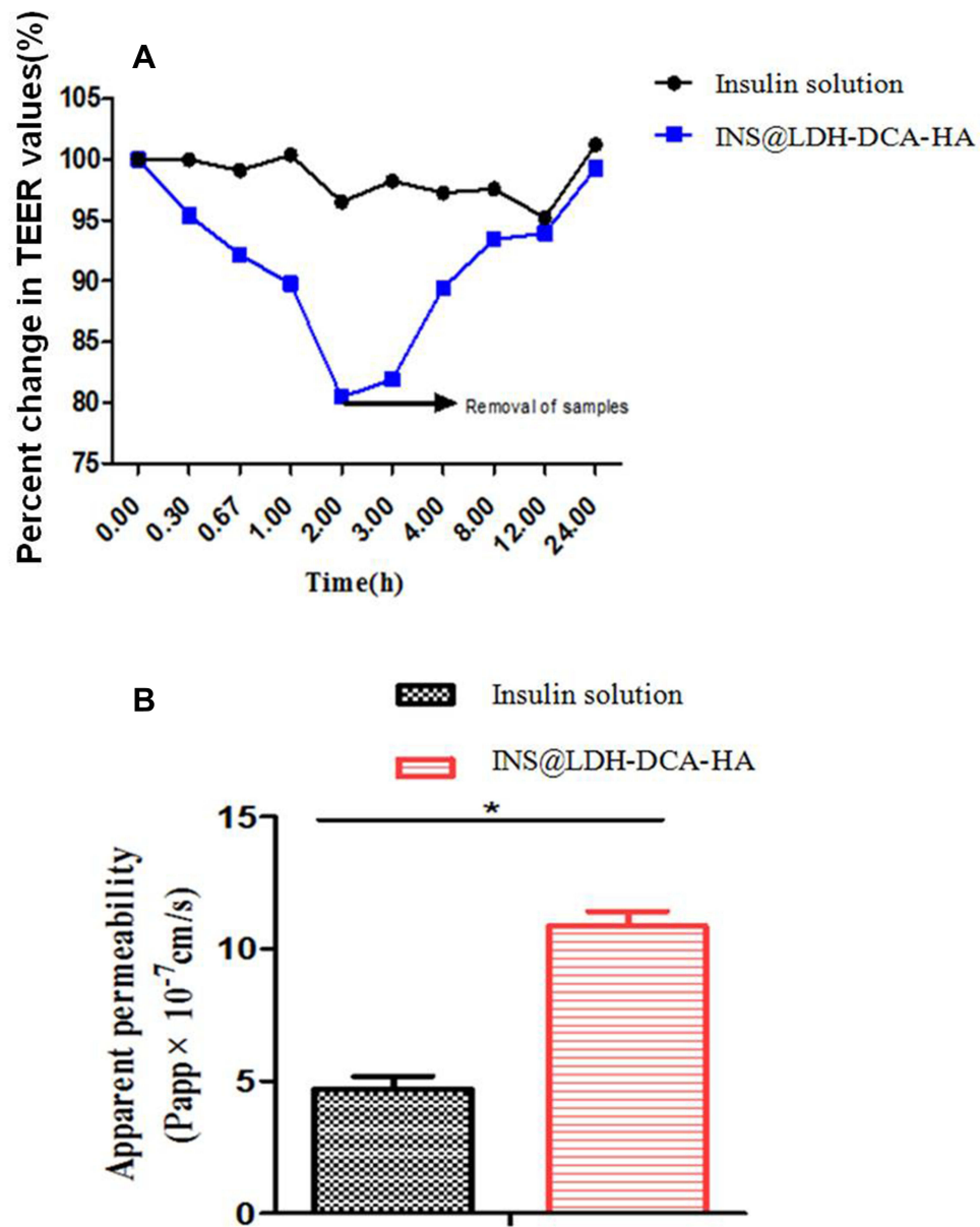
Figure 7 Transepithelial transport of insulin. (A) Effects of insulin solution and INS@LDH-DCA-HA NPs on transepithelial transport of Caco-2 cell monolayer. (B) Apparent permeability coefficient (Papp) of insulin across Caco-2 monolayer with incubation for 2 h. *P < 0.05.
