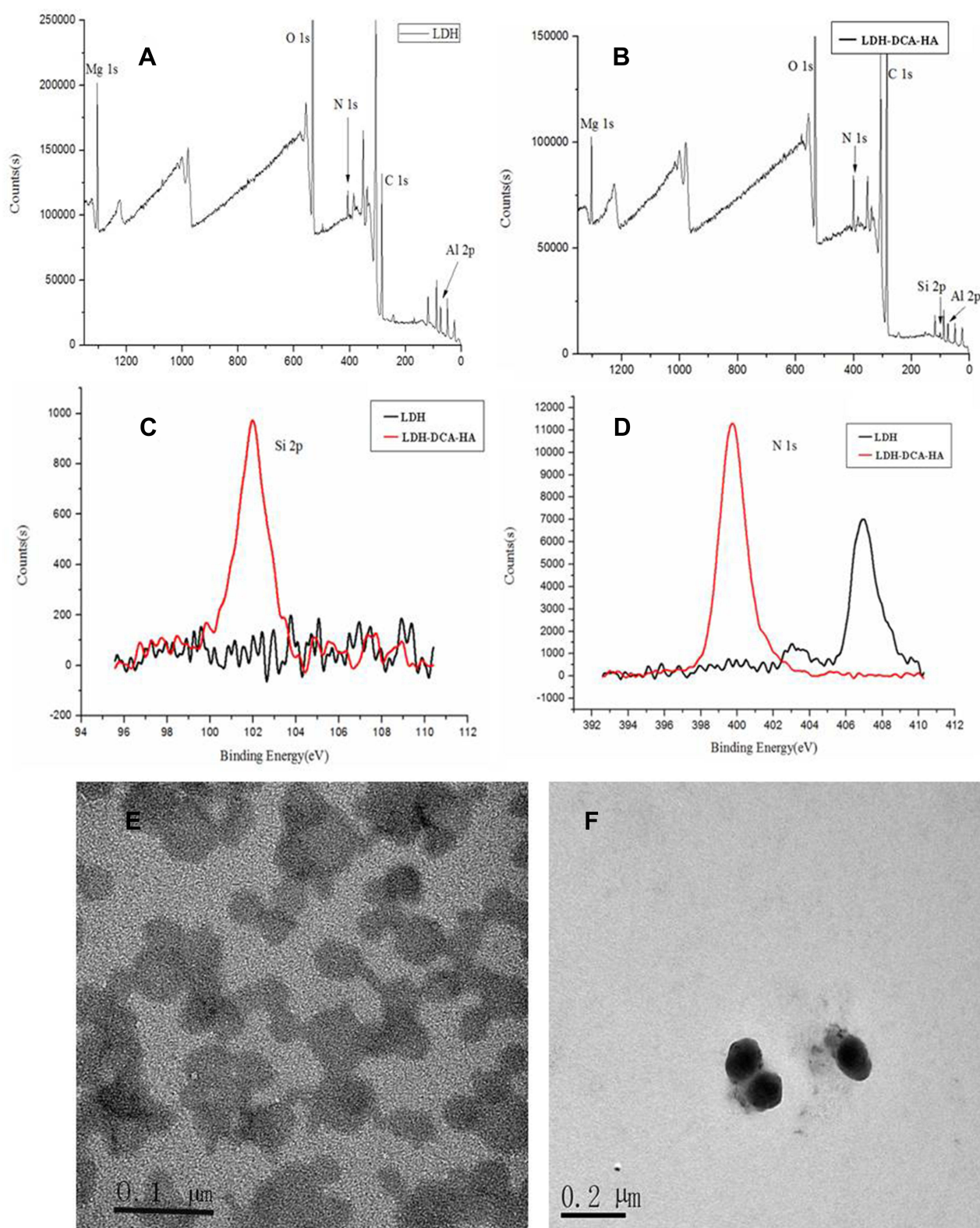
Figure 1 X-ray photoelectron spectroscopy analysis of LDH and LDH-DCA-HA. (A–D); morphology of LDH (E) and LDH-DCA-HA (F) by TEM.
