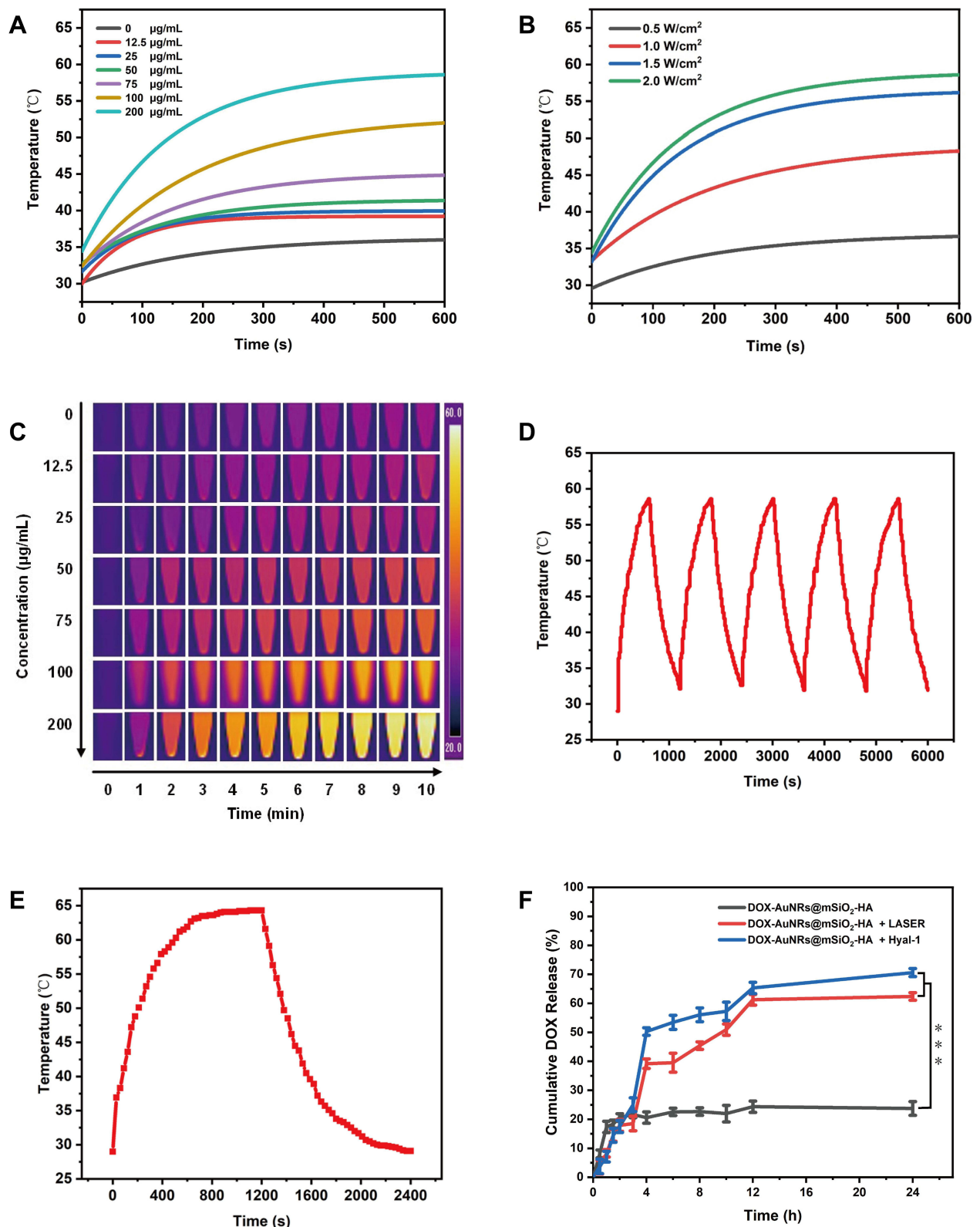
Figure 3 Temperature-rising assessment and drug release of AuNRs@mSiO 2 -based nanocomposites. (A) Temperature change of the AuNRs@mSiO 2 -HA aqueous solution under NIR laser irradiation (2.0 W cm -2 , 808 nm). (B) Temperature elevation in the AuNRs@mSiO 2 -HA aqueous solution (1.0 mL, 200 µg mL -1 ) with NIR laser exposure as a function of power density. (C) IR thermographic maps of the cavities containing AuNRs@mSiO 2 -HA aqueous solution subjected to 10 min of NIR irradiation (2.0 W cm -2 , 808 nm). (D) Temperature evolution of AuNRs@mSiO 2 -HA aqueous solution (1.0 mL, 200 µg mL -1 ) over five lasers ON/OFF cycles of NIR laser irradiation (2 W cm -2 , 808 nm). (E) The photothermal response of AuNRs@mSiO 2 -HA aqueous solution (1.0 mL, 200 µg mL -1 ) exposed by NIR laser (2.0 W cm -2 , 808 nm) until reaching a stabilized temperature and then the laser was turned off. (F) DOX release profiles from DOX-AuNRs@mSiO 2 -HA in PBS at different pH values. Data are expressed as mean ± S D (n = 3). ***P < 0.001.
