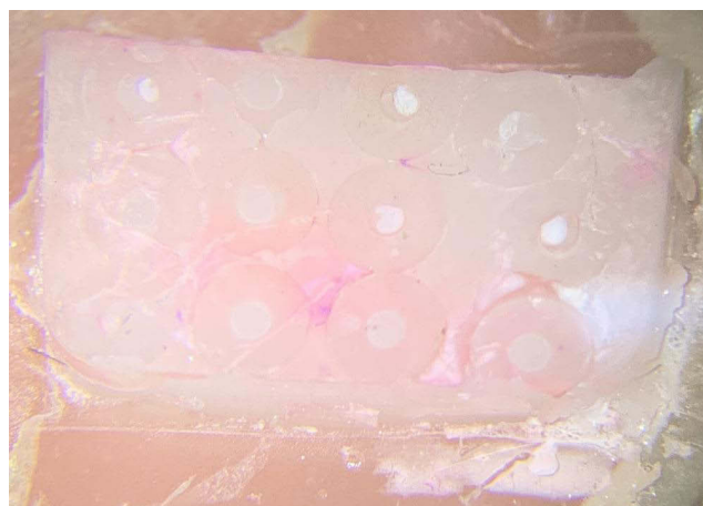
Figure 5 Failure adhesive/mixed.
