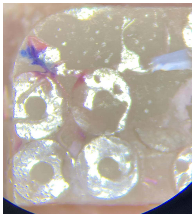
Figure 4 Failure cohesive in ceramic.
