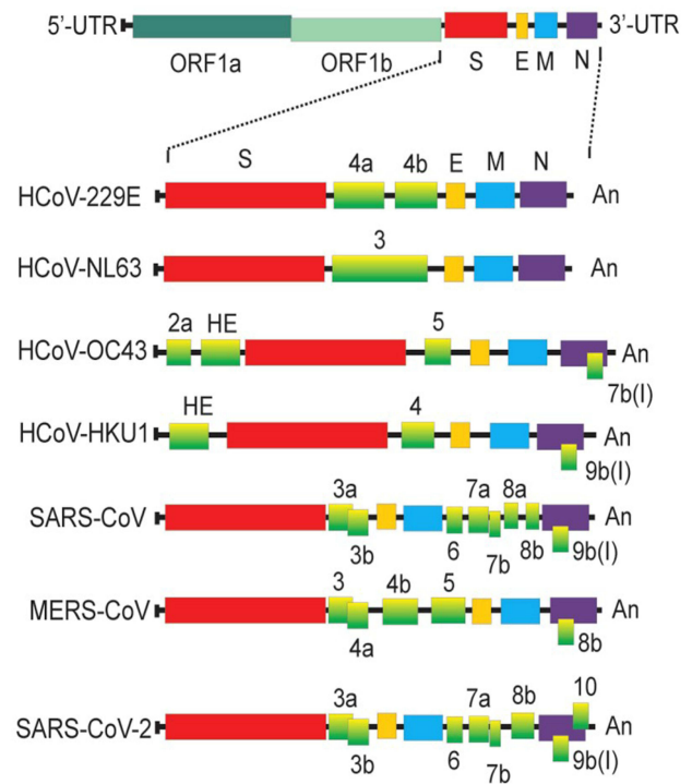
Figure 4 Comparison of different genome structures of coronaviruses.
