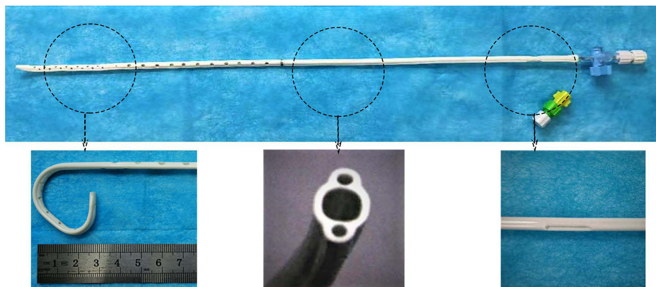
Figure 1 A novel brachytherapy biliary drainage catheter (BBDC).
