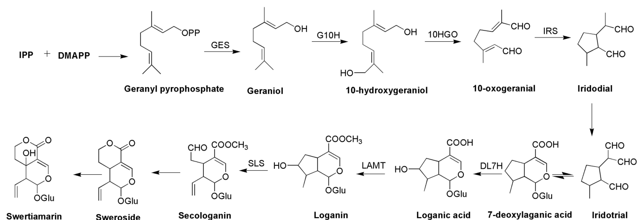
Figure 6 Biosynthetic pathway of swertiamarin (seco-iridoid pathway).
