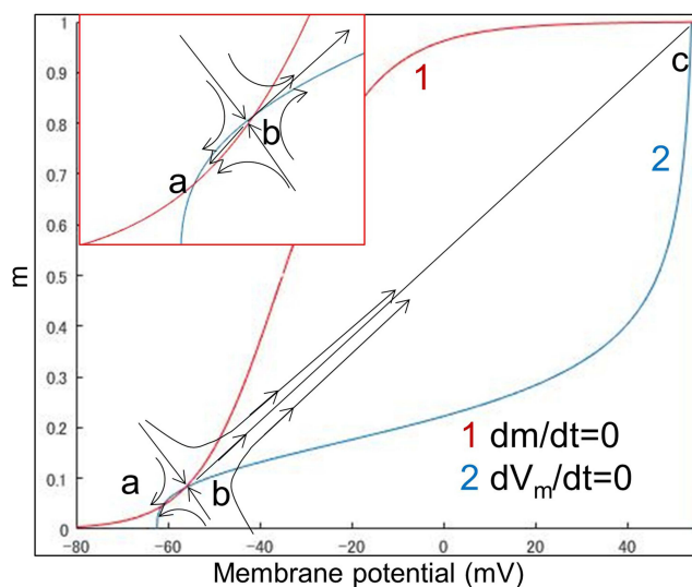
Figure 3 An example of the phase portrait of the C-fiber model. The figure shows the dynamic.
