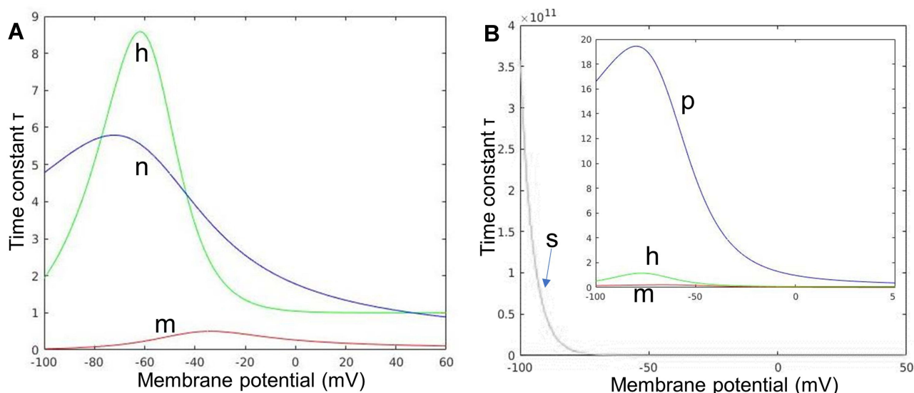
Figure 2 The time constants of each ion channel in the C(A) and Aδ(B) models.
