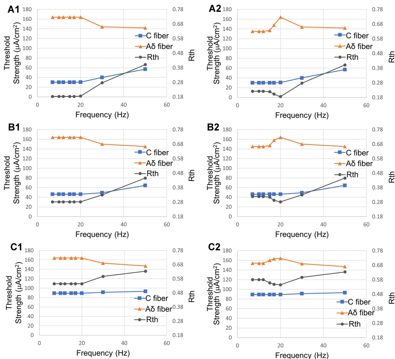
Figure 14 Relationship between pulse frequency, threshold strength, and R_{th} over PAR. (A1 and A2) PAR with 1:6, (B1 and B2) PAR with 1:3, (C1 and C2) PAR with 1:1. The threshold strength of the C-fiber model increases, and that of the A \delta -fiber model decreases after 20 Hz. According to the change in R_{th} over frequency, a lower frequency amplifies PAR's effects.
