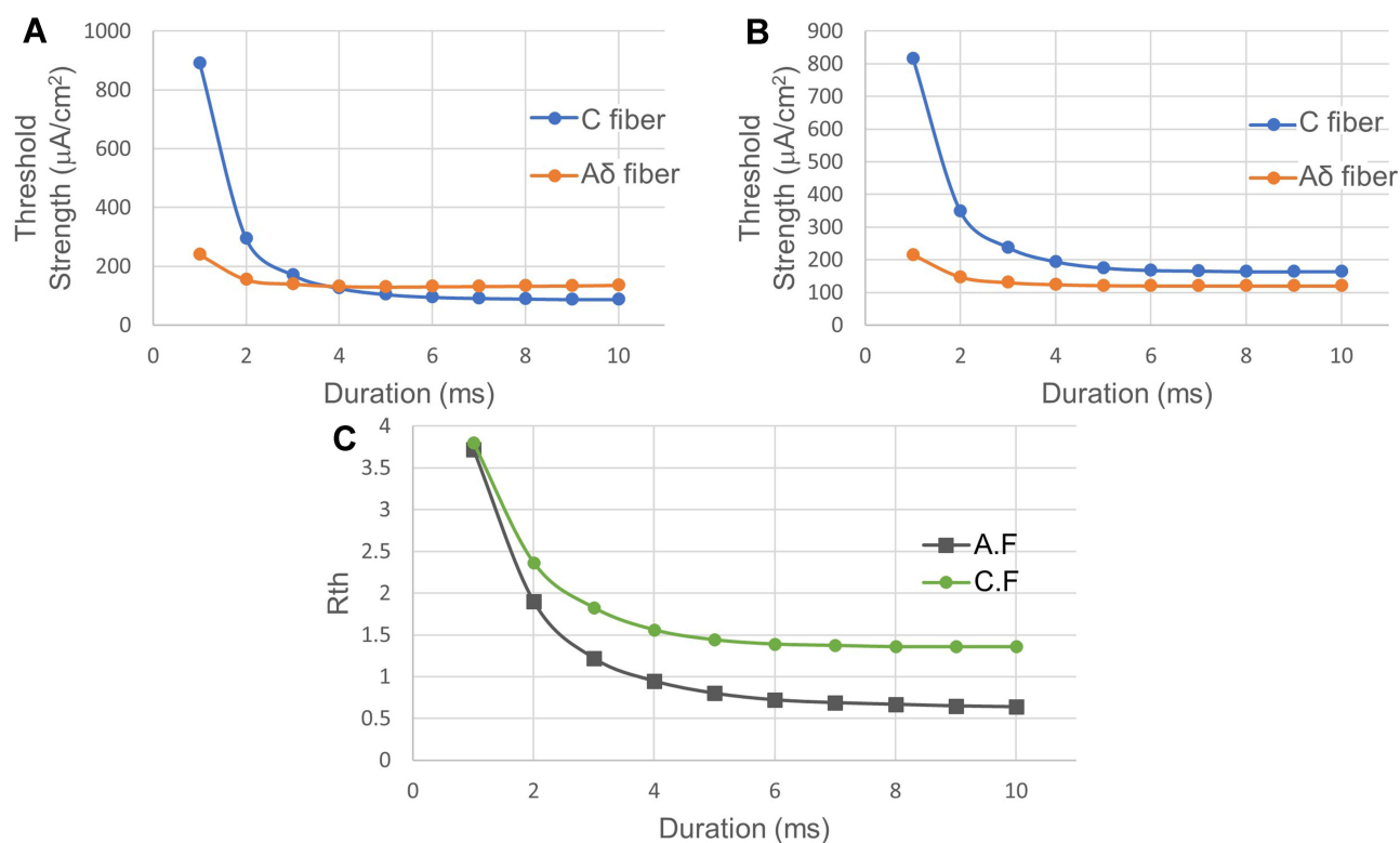
Figure 10 Stimulation with biphasic symmetrical waveforms with different durations. (A) Anodal stimulus before cathodal stimulus (A.F.). (B) Cathodal stimulus before anodal stimulus (C.F.). (C) The threshold ratio between the C-fiber model and Aδ-fiber model ( R_{th} ) with different duration values. In A.F. stimulation case, the threshold strength of the C-fiber model turns lower than that of the Aδ-fiber model when the duration is longer than 4 ms, but this does not occur in C.F. stimulation case. That is, the A.F. stimulation gives positive feedback on C-selectivity.
