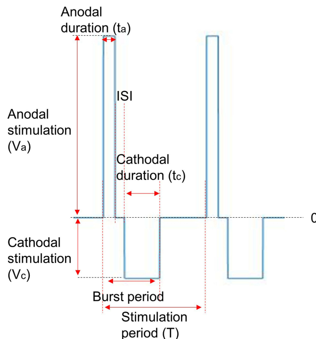
Figure 4 An example of the stimulation waveform.
