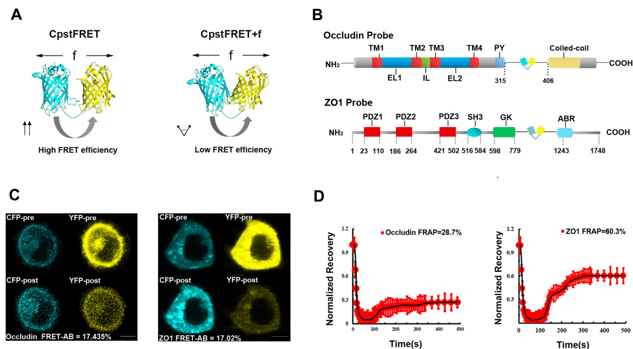
Figure 1 Construction of occludin/ZO1 probes and analysis of their efficacy and motility. (A) In cpsstFRET (cpVenus-7aa-cpCerulean), cpCerulean (cyan) is the donor and cpVenus (yellow) is the acceptor. The probes have high Förster resonance energy transfer (FRET) efficiency when donor and acceptor are parallel without external force (f: external force). The external force reduces the FRET efficiency by changing the angle of cpsstFRET. (B) Schematic representation of the occludin/ZO1 probe constructs. The cpsstFRET module was inserted between amino acids 357 and 358 in the occludin probe and between amino acids 1011 and 1012 in the ZO1 probe. (C) FRET acceptor photobleaching (FRET-AB) was used to test the efficacy of the occludin (left) and ZO1 (right) probes in HBMEC cells. FRET-AB efficiency was 17.435% for the occludin probe and 17.02% for the ZO1 probe. (D) The intracellular mobility of the occludin (left) and ZO1 probes (right) were determined using fluorescence recovery after photobleaching (FRAP). The normalized average fluorescence recovery of occludin (left) and ZO1 (right) vs time (500 s) was calculated (n = 8), and the fluorescence recovery ratio noted. Scale bar: 20 \mu m.
