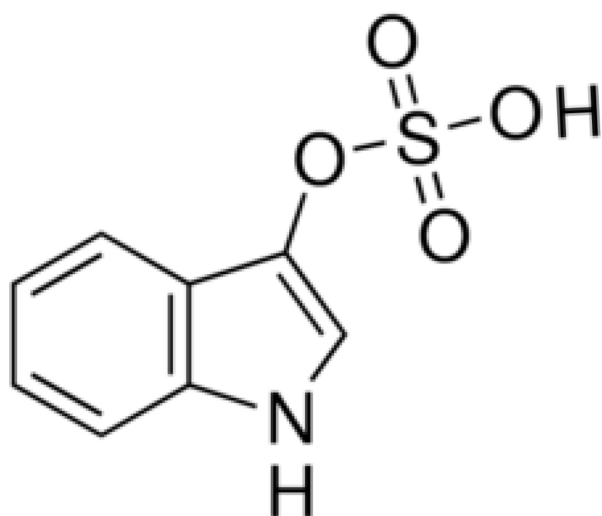
Figure 1 Structure of indoxyl sulfate: C_8H_7NO_4S .
