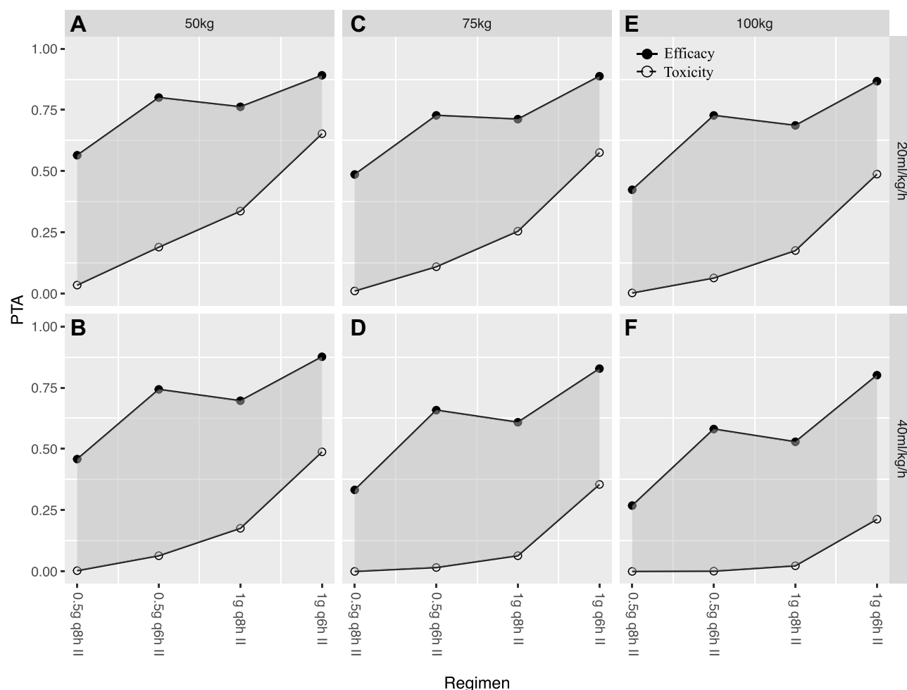
Figure 5 Probability of target attainment (PTA) for a MIC of 1 mg/L when efficacy is defined as 100% fT > MIC and toxicity is defined as an C_{min} > 10 mg/L for imipenem doses administered to critically-ill patients during CRRT: (A) dosing schedule for critically-ill patients weighing 50 kg in CRRT intensity of 20 mL/kg/h; (B) dosing schedule for critically-ill patients weighing 50 kg in CRRT intensity of 40 mL/kg/h; (C) dosing schedule for critically-ill patients weighing 75 kg in CRRT intensity of 20 mL/kg/h; (D) dosing schedule for critically-ill patients weighing 75 kg in CRRT intensity of 40 mL/kg/h; (E) dosing schedule for critically-ill patients weighing 100 kg in CRRT intensity of 20 mL/kg/h; (F) dosing schedule for critically-ill patients weighing 75 kg in CRRT intensity of 40 mL/kg/h.
