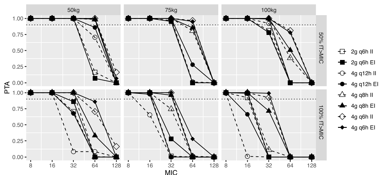
Figure 2 Probability of target attainment (PTA) of 50% or 100% fT > MIC for the piperacillin dosing regimens of 2g q6h, 4g q12h, 4g q8h and 4g q6h in critically ill virtual patients with the CRRT intensity of 35–45 mL/kg/h. II, intermittent infusion as 0.5-h infusion; EI, extended infusion as 4-h infusion. Abbreviation: CRRT, continuous renal replacement therapy.
