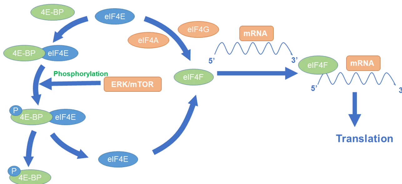
Figure 2 MTOR-mediated synthesis of HIF-1 \alpha .
