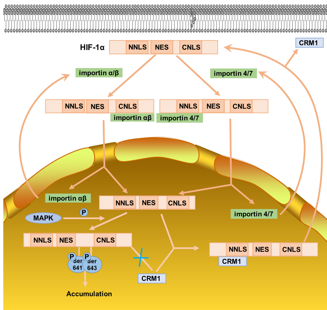
Figure 4 Nuclear transport of HIF-1α.
