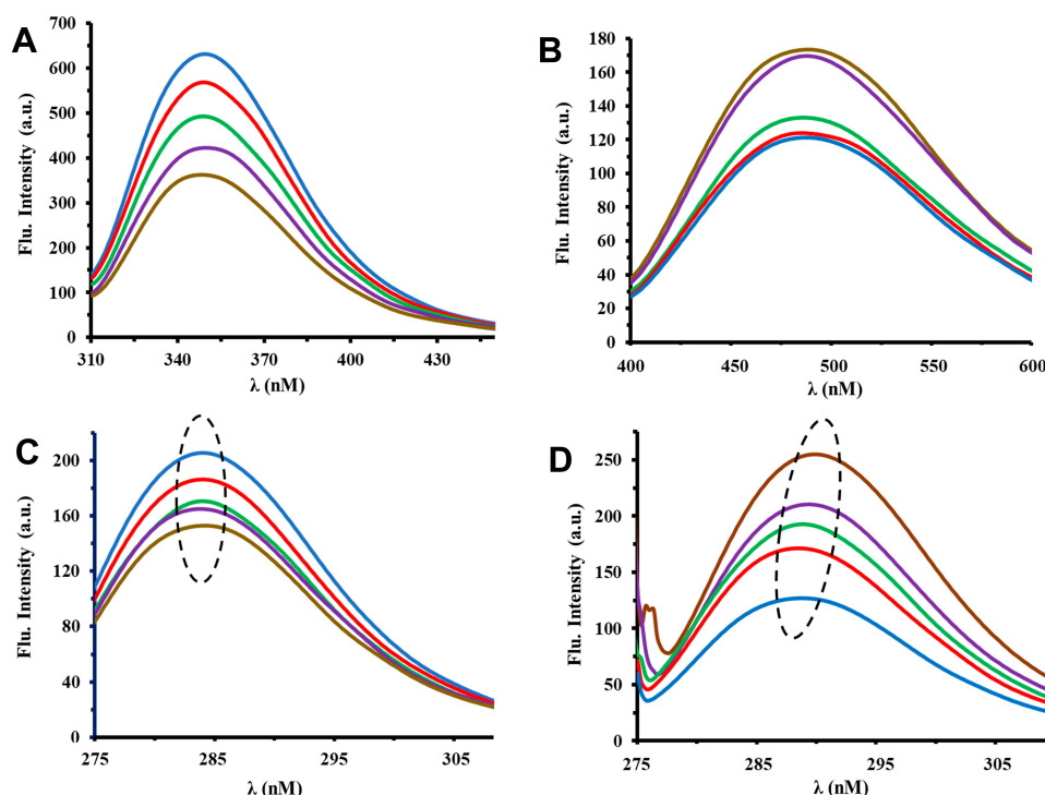
Figure 2 (A) Intrinsic fluorescence, (B) ANS fluorescence, (C) synchronous fluorescence study at \Delta\lambda = 60 nm, and (D) synchronous fluorescence study at \Delta\lambda = 20 nm of HSA after interaction with different concentrations [0 \mu\text{g/mL} (blue), 1 \mu\text{g/mL} (red), 10 \mu\text{g/mL} (green), 20 \mu\text{g/mL} (purple), 50 \mu\text{g/mL} (brown)] of \text{Co}_3\text{O}_4 NPs. The dotted circle shows the red or blue shift in the \lambda_{\text{max}} .
