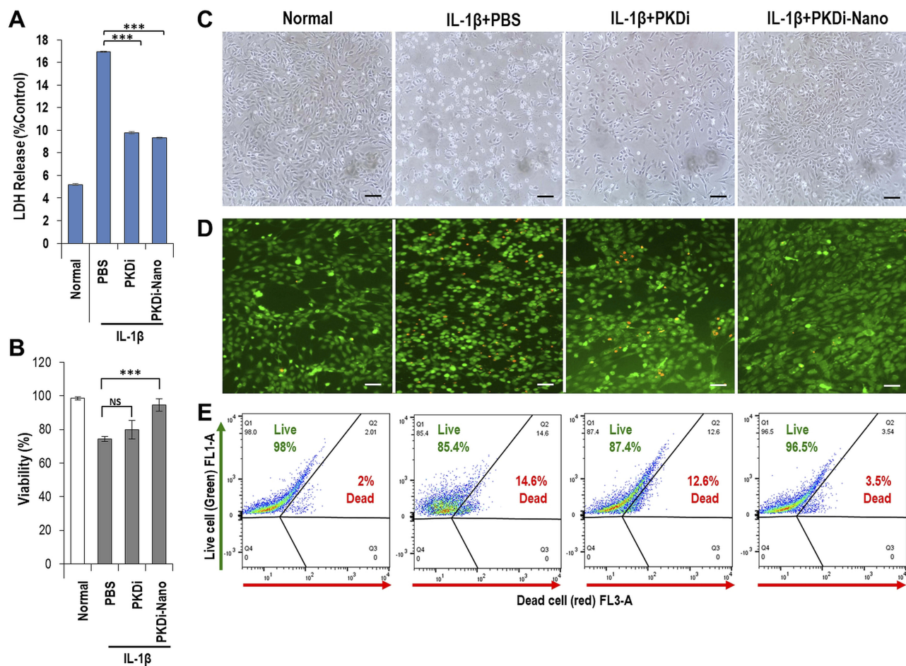
Figure 1 Cytotoxicity, cellular morphology, and viability. (A) Graphical representation of LDH release in the medium. Data are represented as mean \pm SD ( n=5 ). *** P < 0.001 vs PBS, (B) Trypan blue exclusion assay showing percentage of live cells. Data are represented as mean \pm SD ( n=5 ). *** P < 0.001 vs PBS, ^{ns}P > 0.05 vs PBS. (C) Morphology of chondrocytes in monolayer culture. Scale bar = 200 \mu m. (D) Live/dead stain fluorescence images. Live cells (green) dead cells (red). Scale bar = 200 \mu m. (E) Flow cytometry analysis after live/dead stain. Percentage of live cells is represented in Q1 and Q2, respectively. Data are represented as mean \pm SD ( n=5 ).
