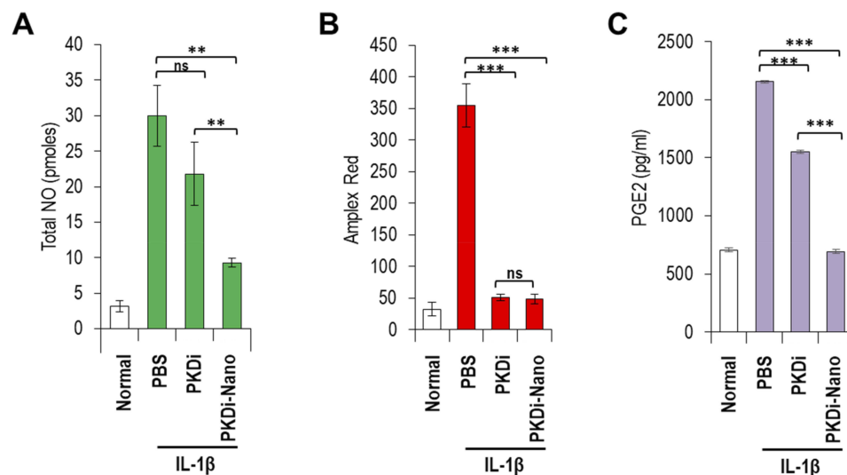
Figure 3 Biochemical analyses of treated chondrocytes. (A) Total NO assay demonstrating reactive nitrogen species. Data are represented as mean concentration (pmole) \pm SD ( n=5 ). ^{**}P < 0.01 vs PBS, ^{ns}P > 0.05 vs PBS. (B) Amplex Red assay indicating reactive oxygen species ( H_2O_2 ). Data are represented as mean concentration (uM) or mean RFU \pm SD ( n=5 ). ^{***}P < 0.001 vs PBS, ^{ns}P > 0.05 vs PKDi. (C) PGE2 assay showing degree of inflammation. Data are represented as mean concentration (pg/ml) \pm SD ( n=5 ). ^{***}P < 0.001 vs PBS.
