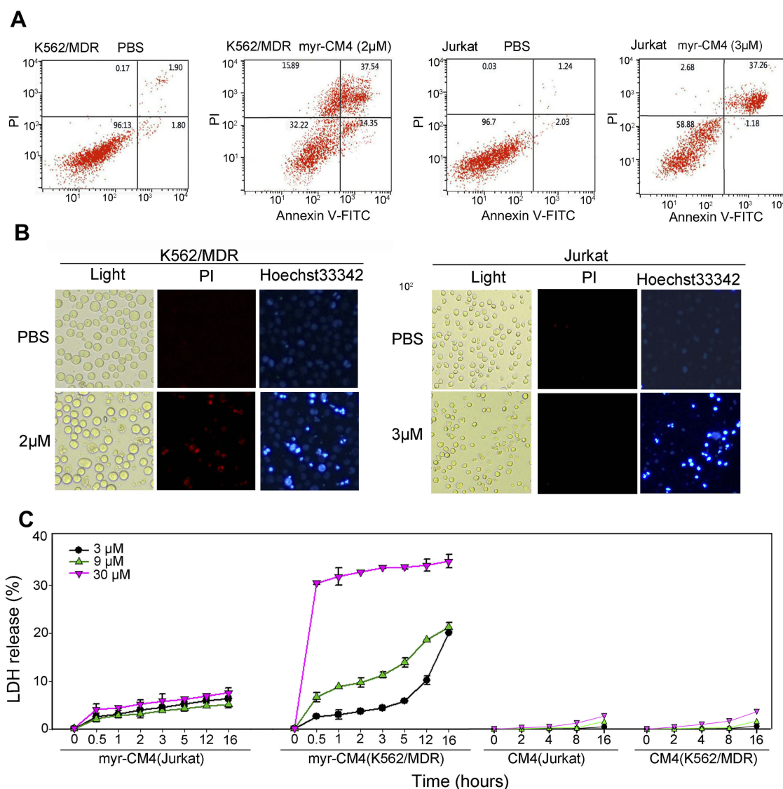
Figure 4 Necrosis and apoptosis of leukemia cells induced by myristoyl-CM4. (A) K562/MDR and Jurkat cells were treated with myristoyl-CM4 (2 \mu M for K562/MDR, 3 \mu M for Jurkat) for 16 hours, stained by Annexin V-FITC/PI, and analyzed by flow cytometry. (B) Cells were stained with Hoechst 33342/PI and then observed by fluorescence microscopy. (C) Membrane permeability changes were determined by monitoring LDH release from cells after incubation with different concentrations of myristoyl-CM4 (0, 3, 9, 30 \mu M) for different times at 37°C. CM4 was used as a control. Results are the mean \pm SEM of four different experiments.
