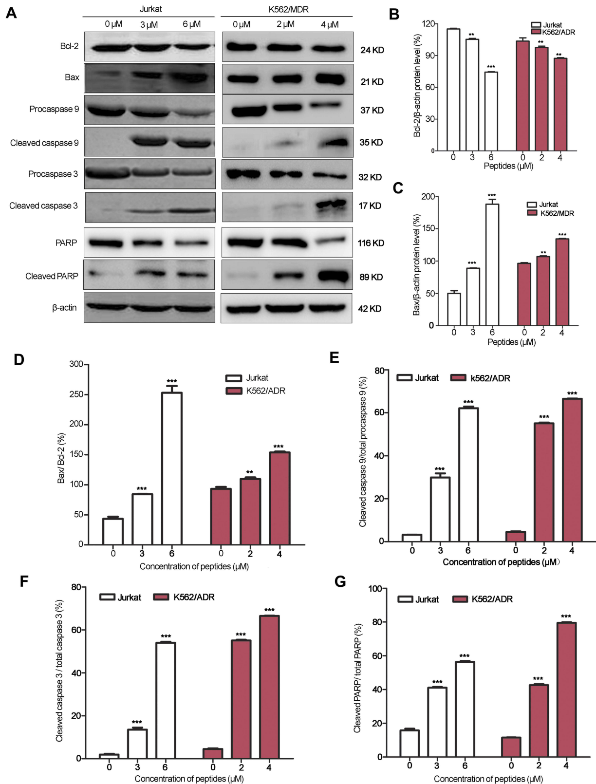
Figure 6 Apoptosis in leukemia cells induced by myristoyl-CM4. (A) Cells were treated with myristoyl-CM4 for 16 hours and the lysates were then harvested and apoptosis-related proteins were detected by Western blotting. The relative amounts of Bax, Bcl-2, active (cleaved) caspase 9, active (cleaved) caspase 3, and cleaved PARP relative \beta -actin control were determined by Western blotting and Image J densitometric analysis. The Bcl2 (B), Bax (C), Bax/Bcl-2 ratio (D), cleaved caspase 9/total caspase 9 ratio (E), cleaved caspase 3/total caspase 3 ratio (F), and cleaved PARP/total PARP ratio (G) were calculated. Results are the mean \pm SEM of three different experiments. ** P < 0.01 ; *** P < 0.001 between PBS control and peptide treatment.
