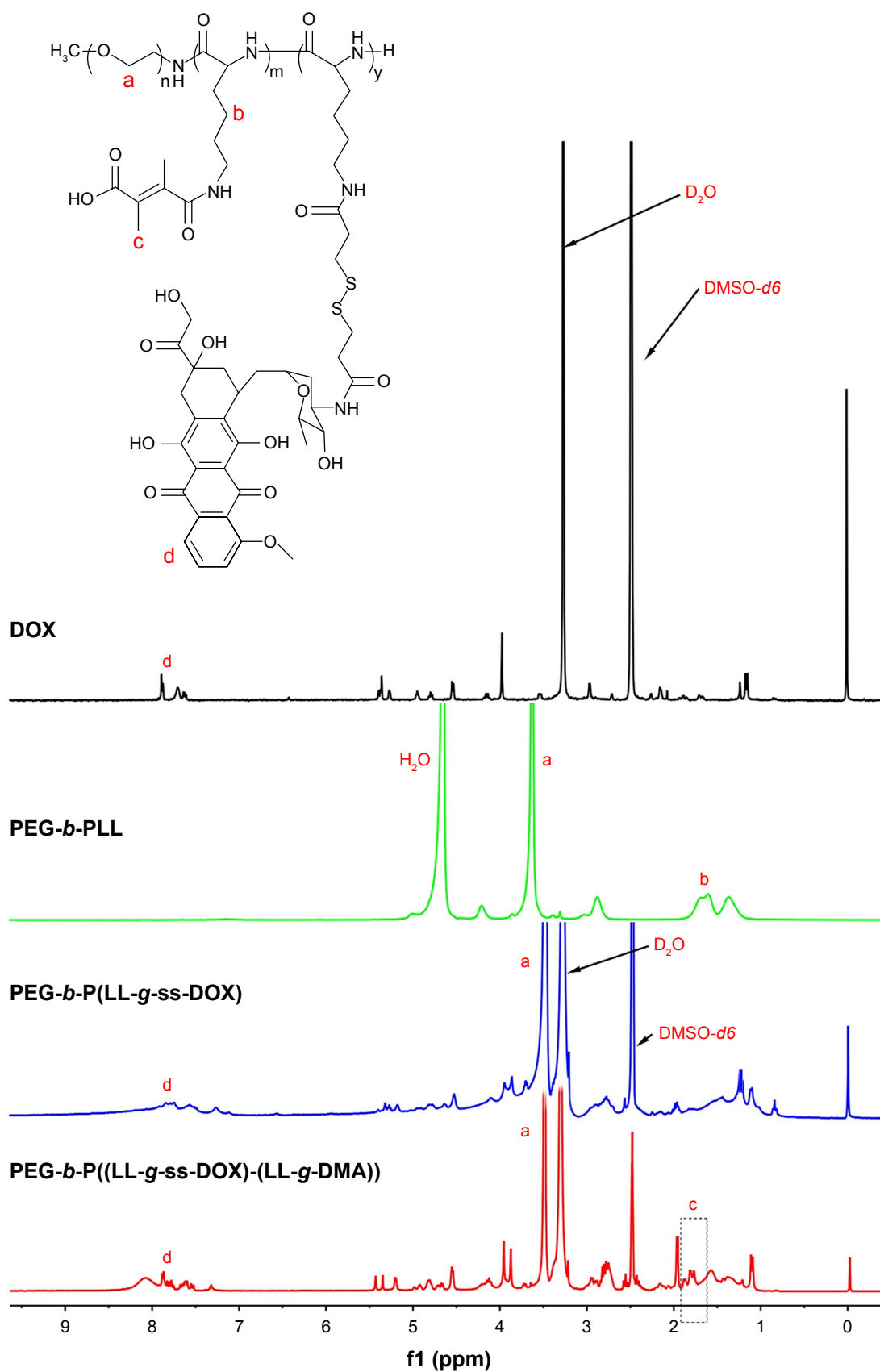
Figure 1 1 H NMR spectra of DOX (in DMSO-d 6 ), PEG-b-PLL (in D 2 O), PEG-b-P(LL-g-ss-DOX) (in DMSO-d 6 ), and PEG-b-P((LL-g-ss-DOX)-(LL-g-DMA)) (in DMSO-d 6 ). Abbreviations: DMSO-d 6 , deuterated dimethyl sulfoxide; DOX, doxorubicin; NMR, nuclear magnetic resonance; PEG-b-PLL, poly(ethylene glycol)-b-poly(L-lysine).
