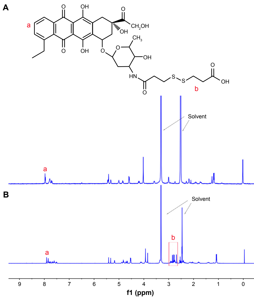
Figure S1 ^1\text{H} NMR spectra of DOX (A) and DTPA-DOX (B) in \text{DMSO}-d_6 .
