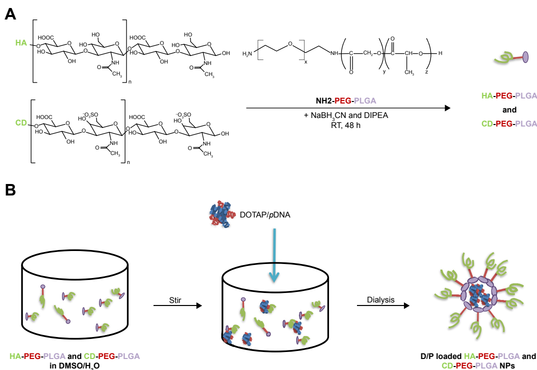
Scheme 1 (A) Synthesis of HA-PEG-PLGA and CD-PEG-PLGA copolymers. (B) Preparation of D/P-loaded NPs.
