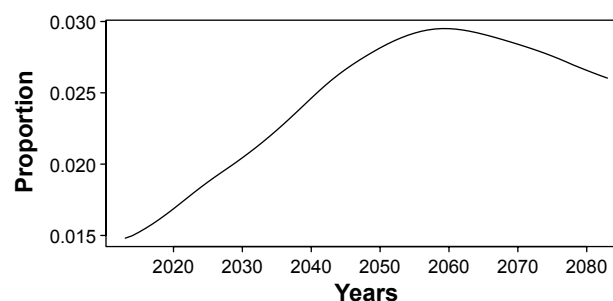
Figure 6 The proportion of patients with Alzheimer's disease to the general population.
