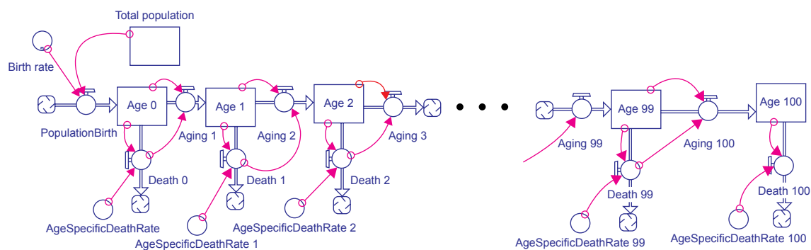
Figure 1 The model of population growth.
