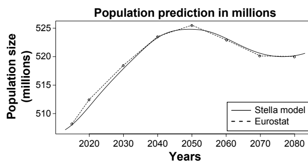
Figure 3 The prediction of population.
