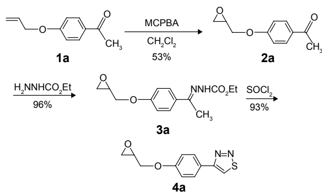
Figure 1 Synthesis of compounds 2a : 4-(1,2-propenoxide-3-yl) acetophenone, 3a : 4-(1,2-Propenoxide-3-yl)acetophenone(ethoxycarbonylhydrazone), 4a : 3-[4-(1,2,3-Thiadiazole-4-yl)phenoxy]-1,2-propenoxide.
