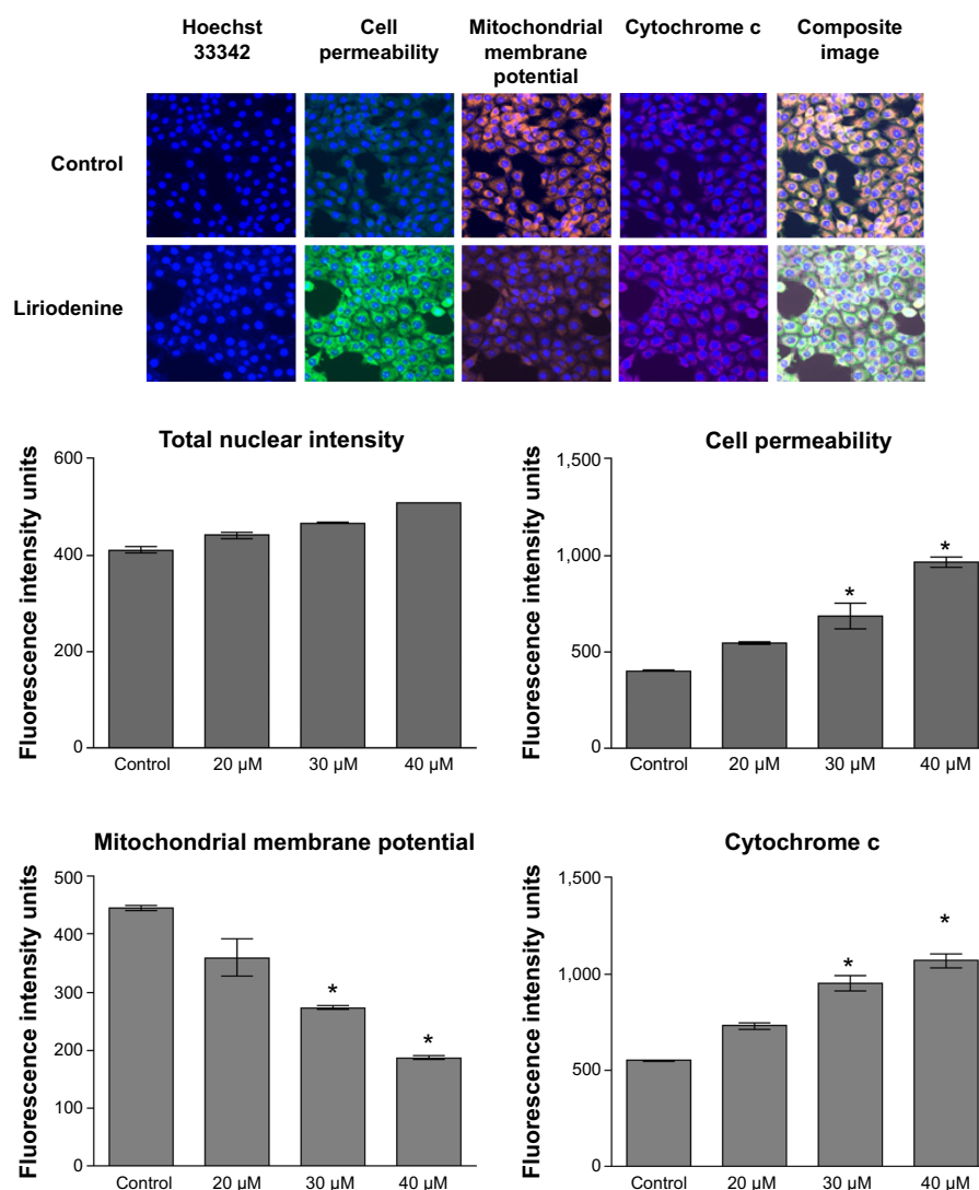
Figure 6 Representative images and quantitative analysis of CAOV-3 cells treated or not treated with liriodenine at 24 hours.
