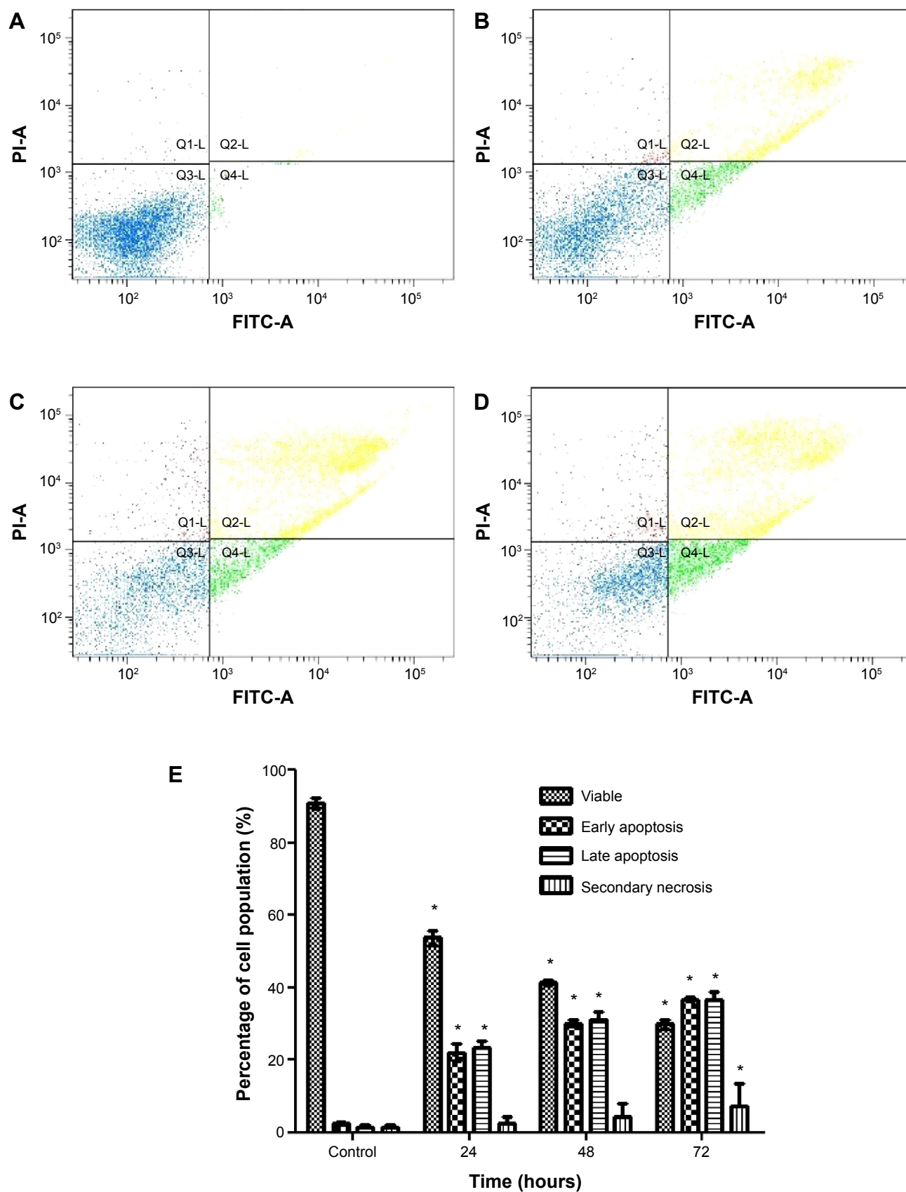
Figure 4 Flow cytometry analysis of Annexin V-fluorescein isothiocyanate in CAOV-3 cells treated with liriodenine in a time-dependent manner.
