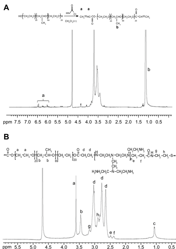
Figure 3 1 H NMR spectra of P123-diacrylate (A) and PA-PEI-SS (B). Note: Lowercase letters (a–h) shown above peaks indicate different proton chemical shifts.
