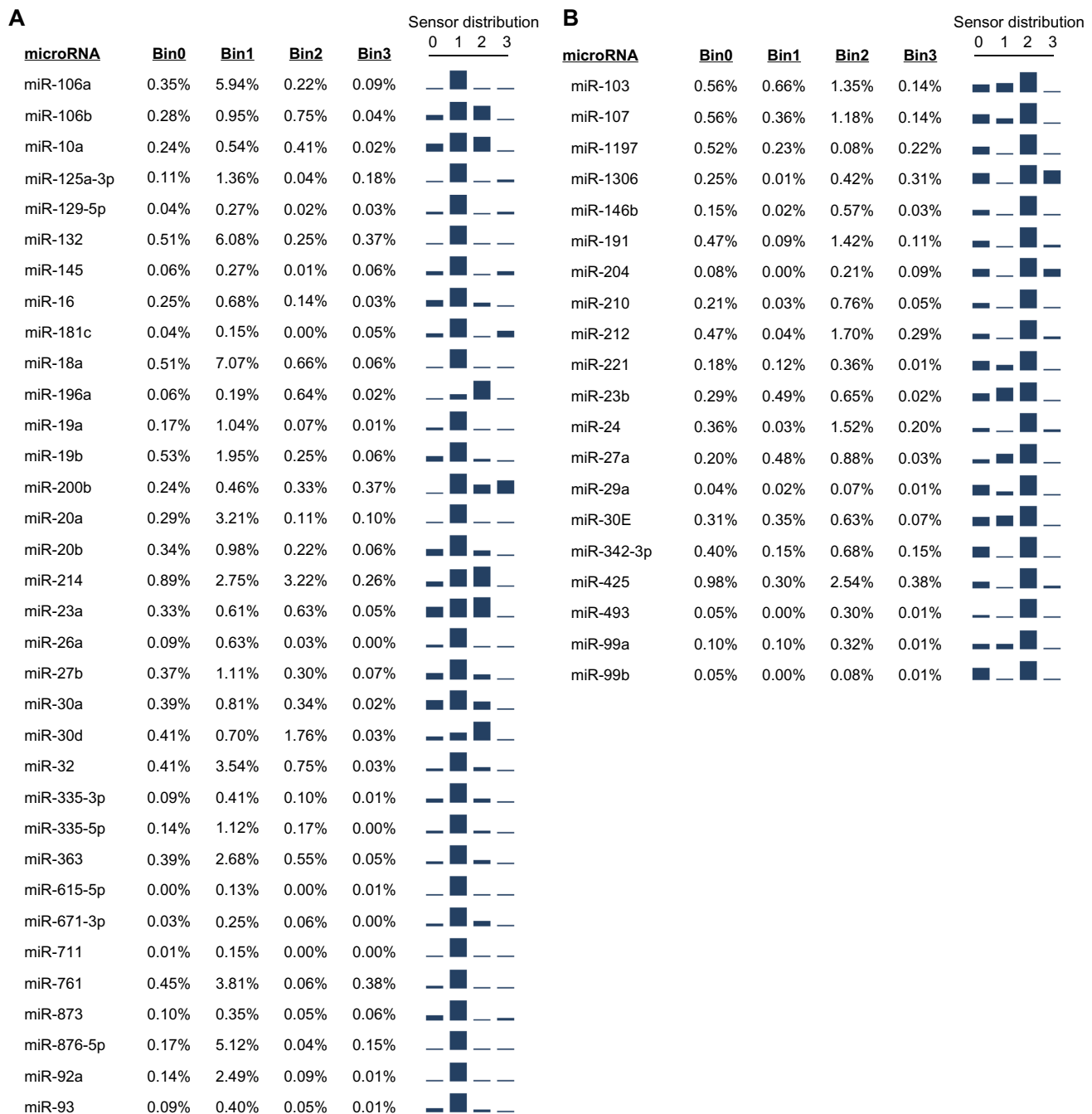
Figure 3 Analysis of target suppression in OVCAR3 cells by Sensor-seq.
