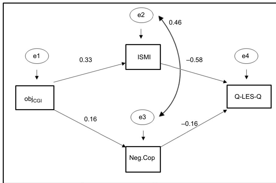
Figure 1 Mediation-analysis model.
