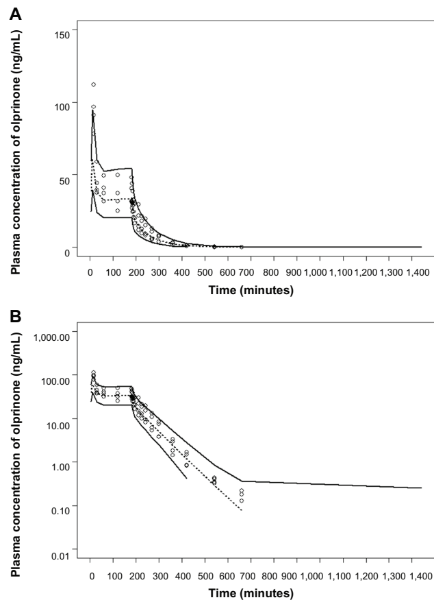
Figure 4 Visual predictive check in the final model for olprinone (Stage VIII, a loading dose at a rate of 1.33 \mu\text{g}/\text{kg}/\text{minute} for 15 minutes followed by continuous infusion at a rate of 0.25 \mu\text{g}/\text{kg}/\text{minute} for 165 minutes).
