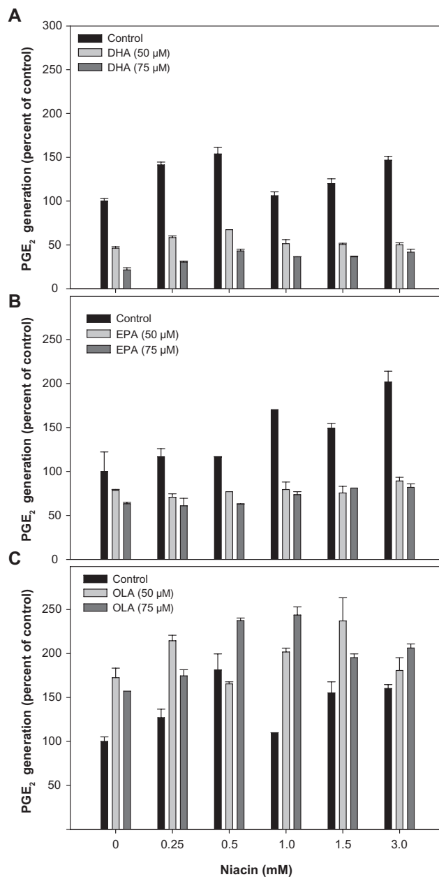
Figure 3 Effect of fatty acids on niacin induced PGE 2 secretion in THP-1 macrophages. Notes: THP-1 macrophages were incubated with 50 and 75 \mu M (A) DHA, (B) EPA, and (C) OLA for 24 hours before being exposed to varying concentrations of niacin for 30 minutes. Concentration of PGE 2 in the medium was determined using an EIA kit as per manufacturer’s instructions (Cayman Chemical, Ann Arbor, MI). Values are the means \pm the standard deviations of duplicate experiments. Abbreviations: DHA, docosahexaenoic acid; EIA, enzyme immunoassay; EPA, eicosapentaenoic acid; PGD 2 , prostaglandin D 2 ; OLA, oleic acid.
