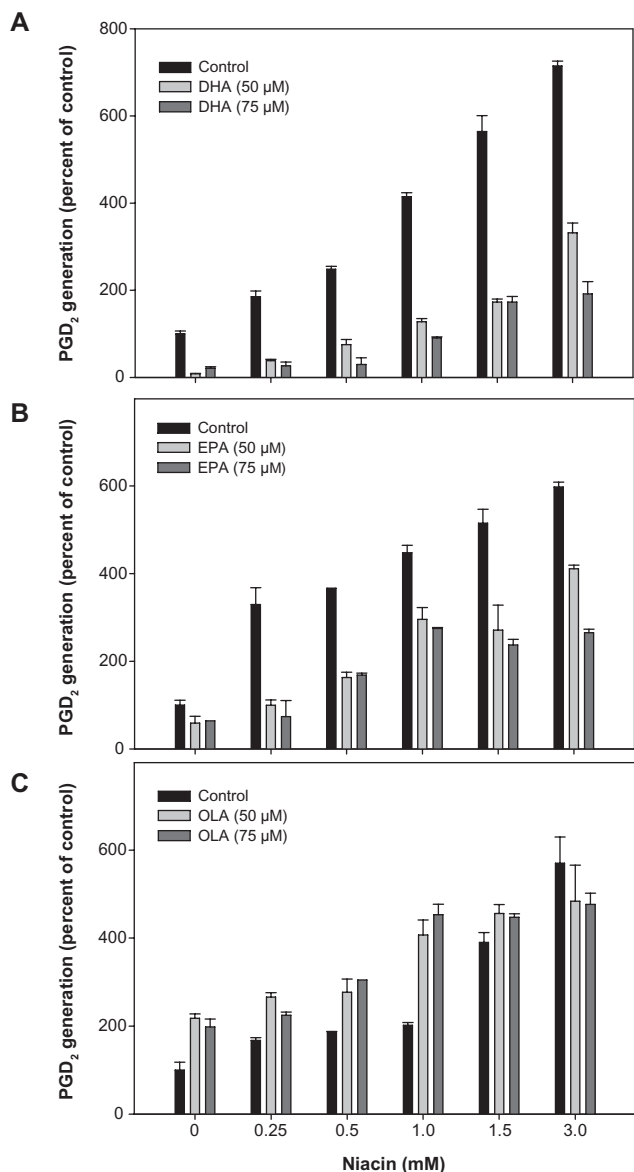
Figure 2 Effect of fatty acids on niacin induced PGD 2 secretion in THP-1 macrophages. Notes: THP-1 macrophages were incubated with 50 and 75 \mu M (A) DHA, (B) EPA, or (C) OLA for 24 hours before being exposed to varying concentrations of niacin for 30 minutes. Concentration of PGD 2 in the medium was determined using an EIA kit as per manufacturer’s instructions (Cayman Chemical, Ann Arbor, MI). Values are the means \pm the standard deviations of duplicate experiments. Abbreviations: DHA, docosahexaenoic acid; EIA, enzyme immunoassay; EPA, eicosapentaenoic acid; PGD 2 , prostaglandin D 2 ; OLA, oleic acid.
