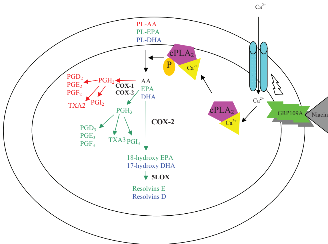
Figure 1 Proposed cellular mechanism for Niacin-induced prostaglandins formation.
