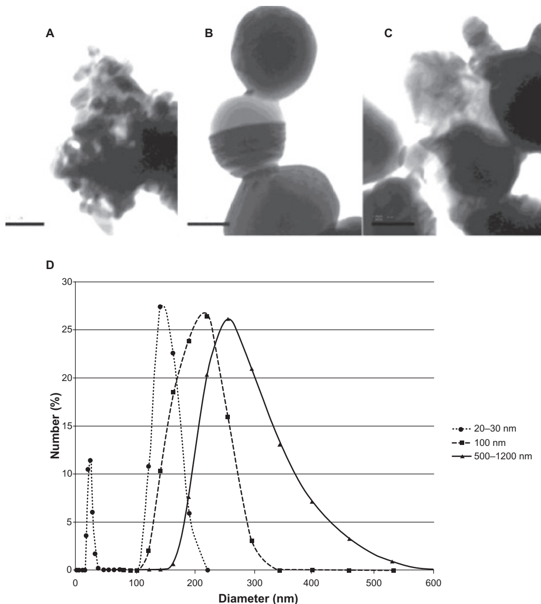
Figure 1 Particle characterization. Transmission electron microscopy images of A ) 20–30 nm, B ) 100 nm, and C ) 500–1200 nm silver particles. D ) Dynamic light-scattering results for the silver nanoparticles.
