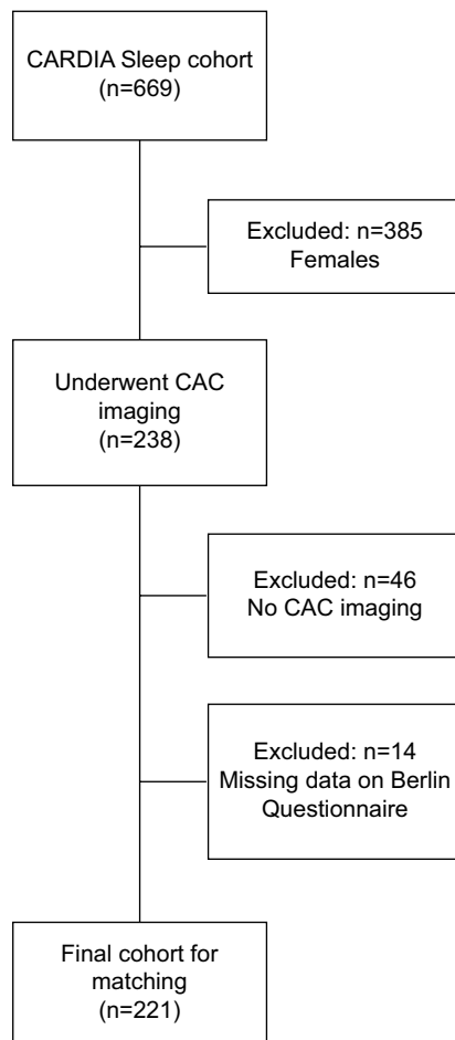
Figure 2 Participant flowchart. Abbreviation: CAC, coronary artery calcium.
