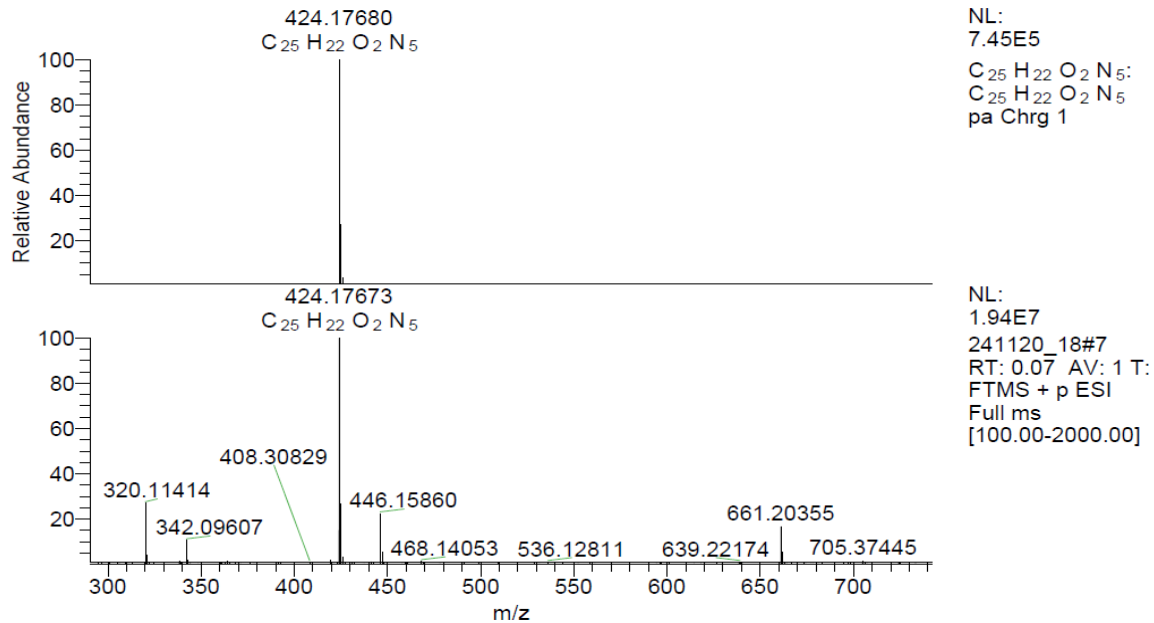
Figure S29. HRMS spectrum of compound 11b
