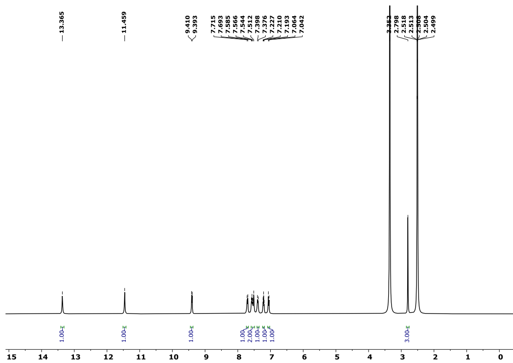
Figure S7. ^1\text{H} NMR (400 MHz, \text{DMSO-}d_6 ) spectrum of compound 5g
