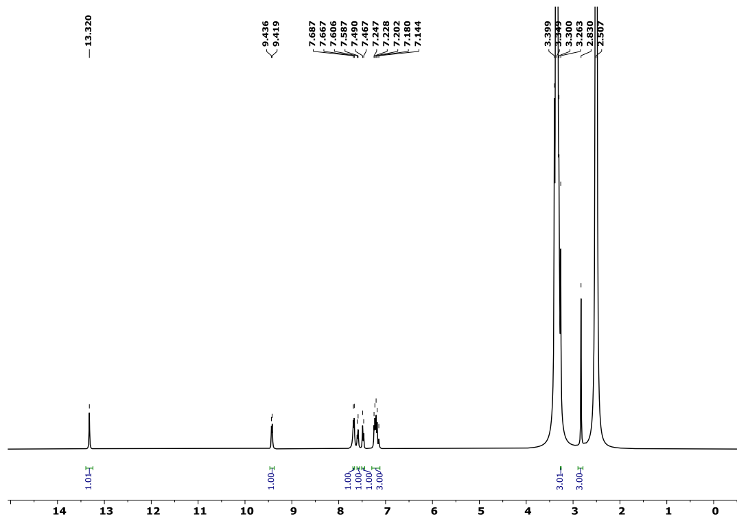
Figure S12. ^1\text{H} NMR (400 MHz, \text{DMSO-}d_6 ) spectrum of compound 8d
