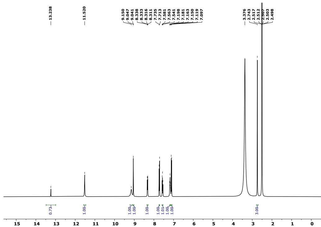
Figure S8. ^1\text{H} NMR (400 MHz, \text{DMSO-}d_6 ) spectrum of compound 5h
