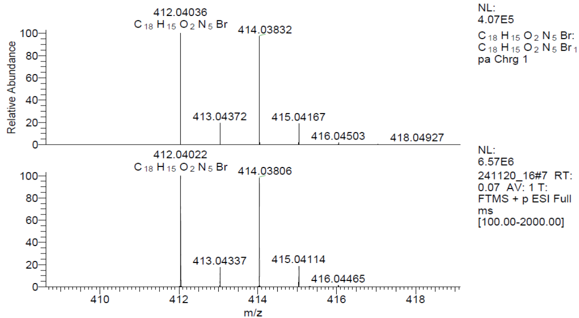
Figure S27. HRMS spectrum of compound 8d
