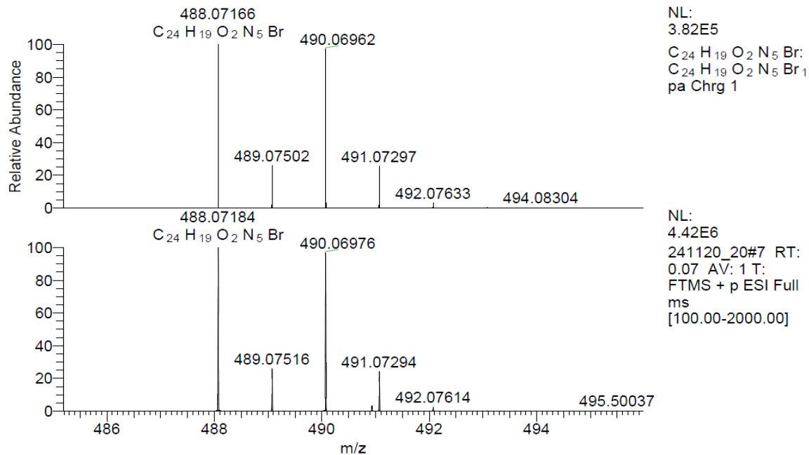
Figure S31. HRMS spectrum of compound 11d
