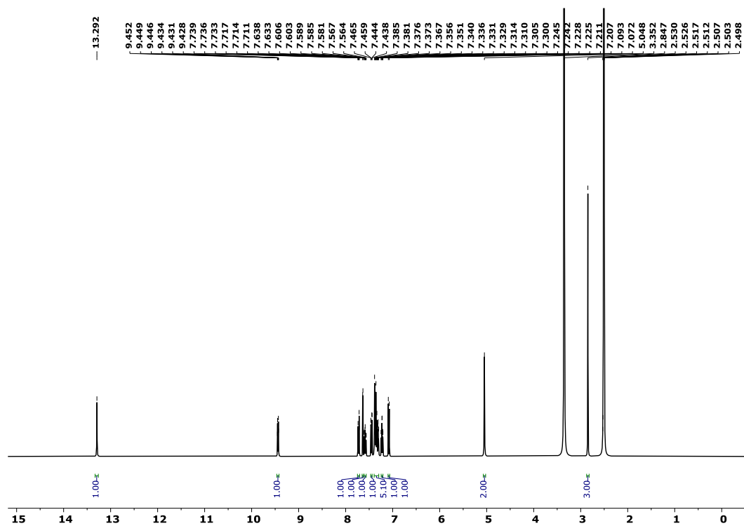
Figure S14. ^1\text{H} NMR (400 MHz, \text{DMSO-}d_6 ) spectrum of compound 11c
