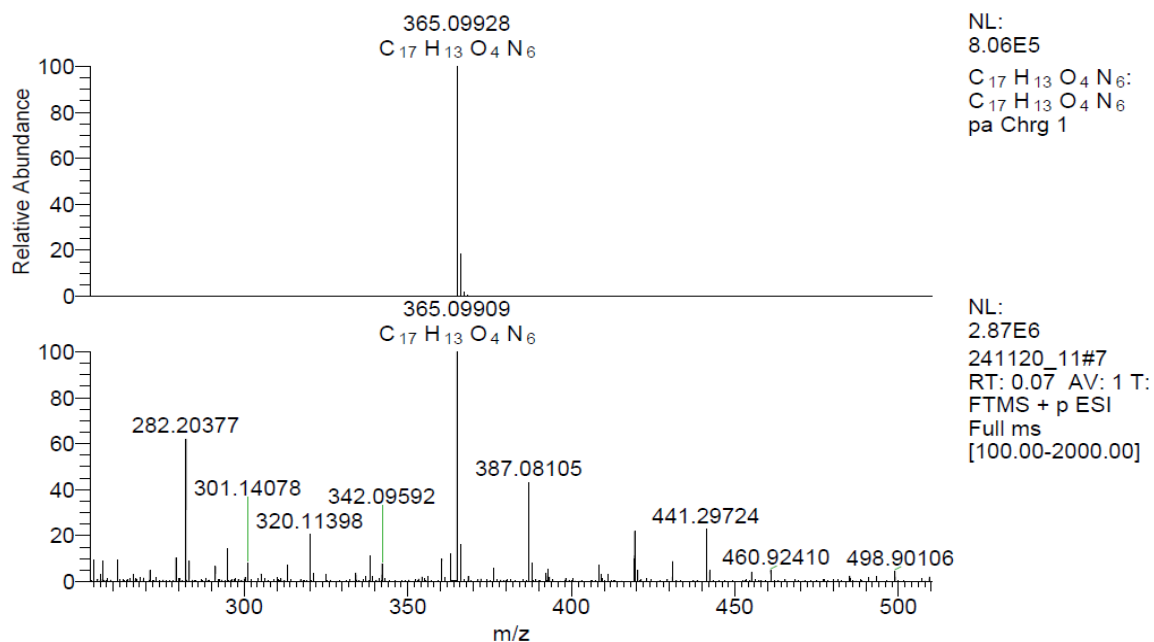
Figure S23. HRMS spectrum of compound 5h
