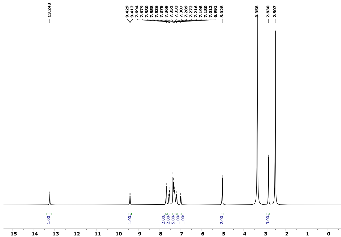
Figure S15. ^1\text{H} NMR (400 MHz, \text{DMSO-}d_6 ) spectrum of compound 11d
