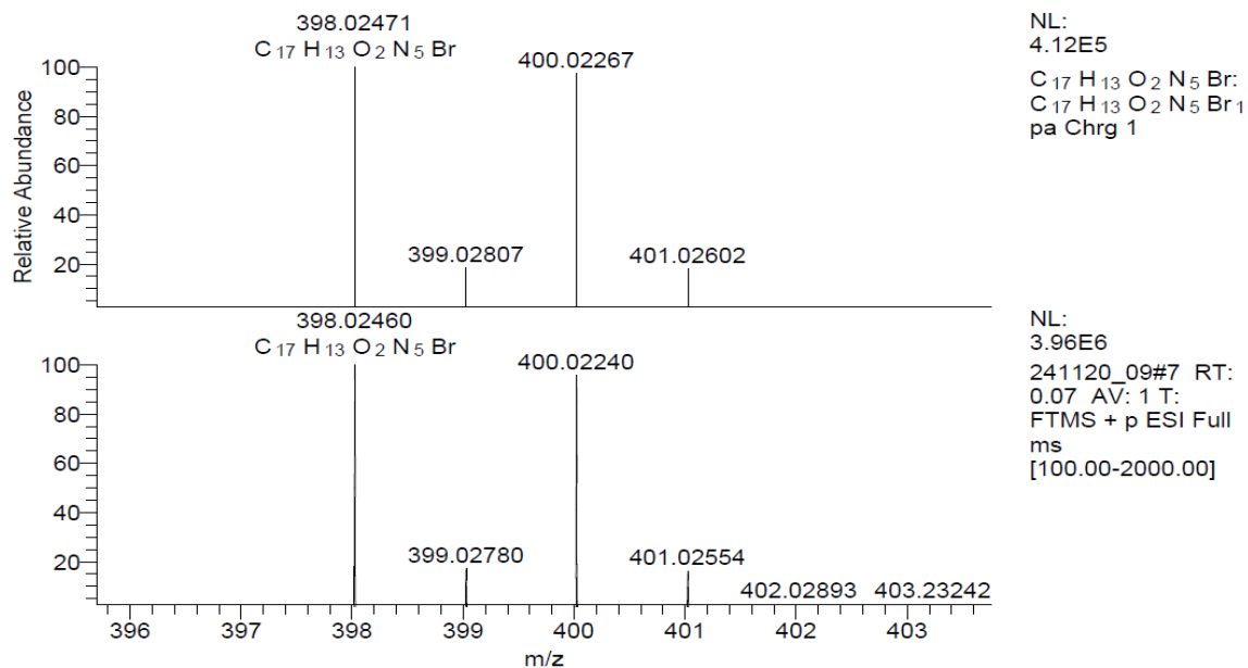
Figure S20. HRMS spectrum of compound 5e
