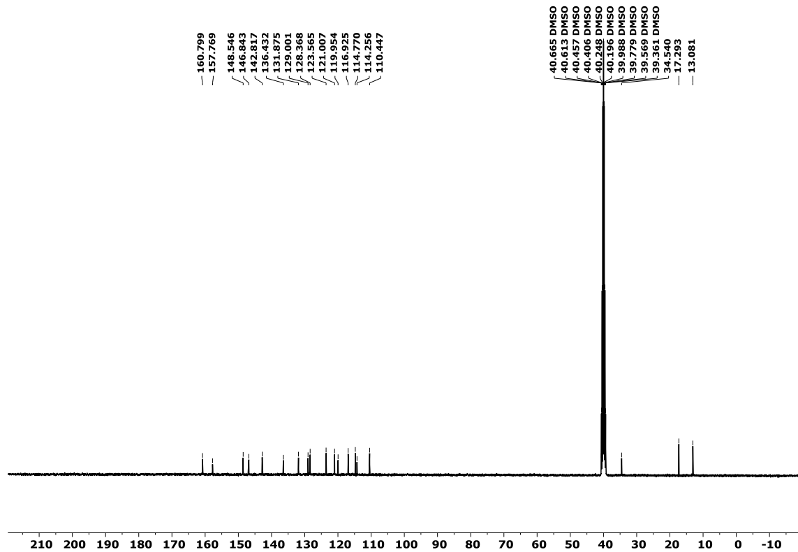
Figure S11. ^{13}\text{C} NMR (100 MHz, \text{DMSO-}d_6 ) spectrum of compound 8b
