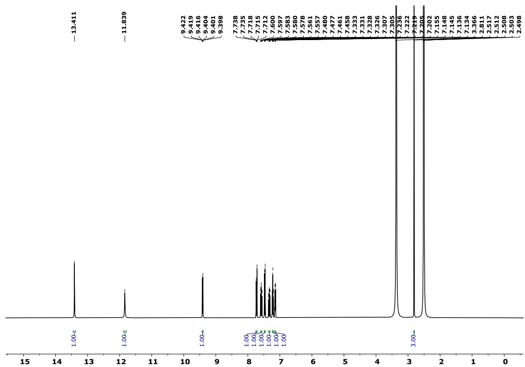
Figure S3. ^1\text{H} NMR (400 MHz, \text{DMSO-}d_6 ) spectrum of compound 5c
