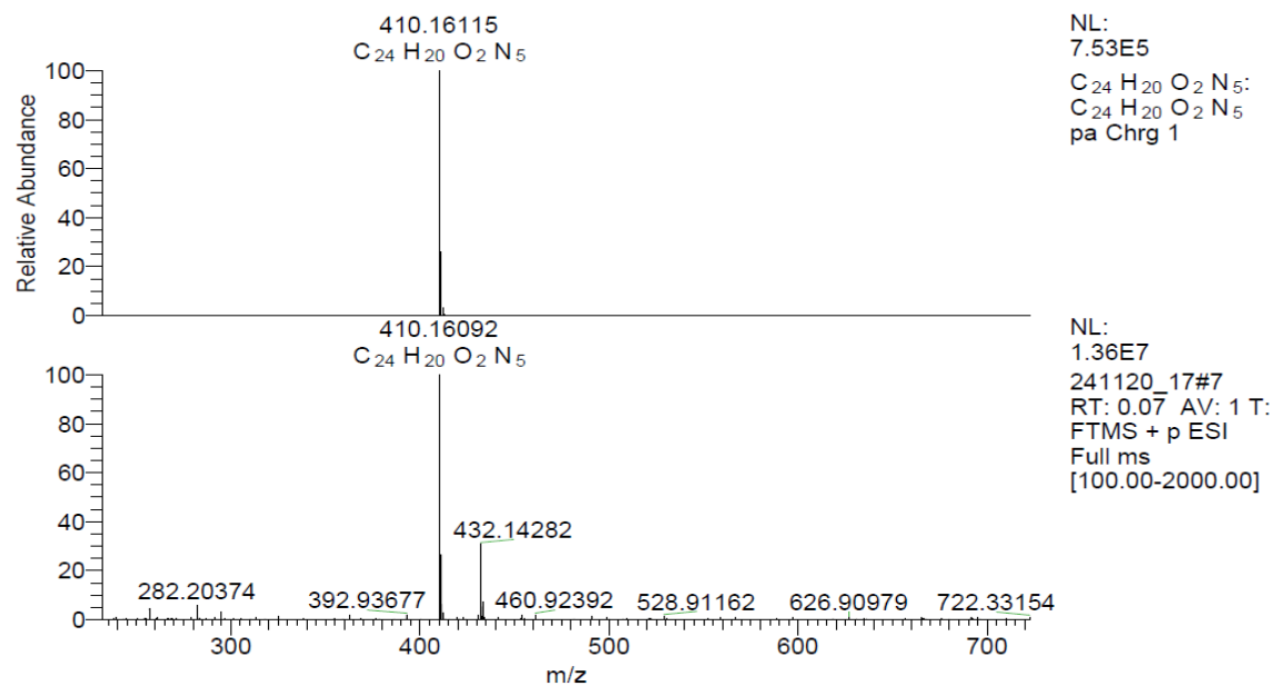
Figure S28. HRMS spectrum of compound 11a
