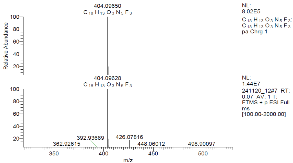
Figure S22. HRMS spectrum of compound 5g
