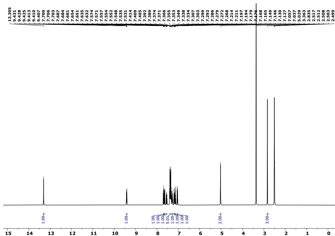
Figure S13. ^1\text{H} NMR (400 MHz, \text{DMSO-}d_6 ) spectrum of compound 11a
