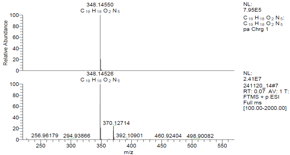
Figure S25. HRMS spectrum of compound 8b
