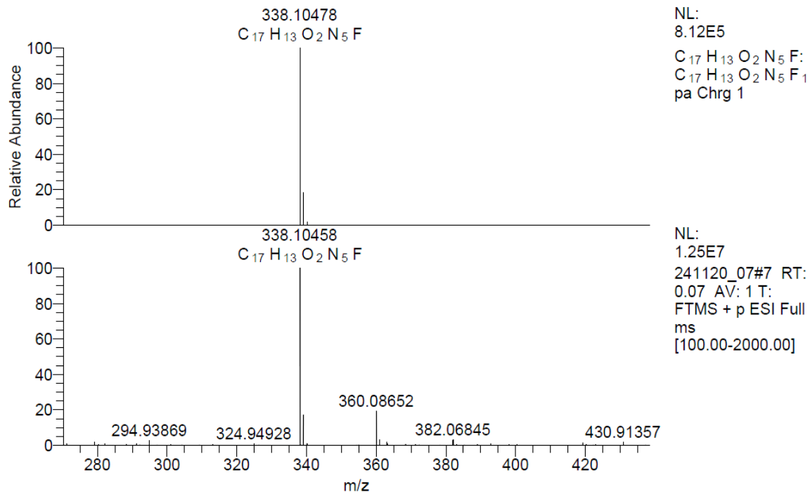
Figure S18. HRMS spectrum of compound 5c
