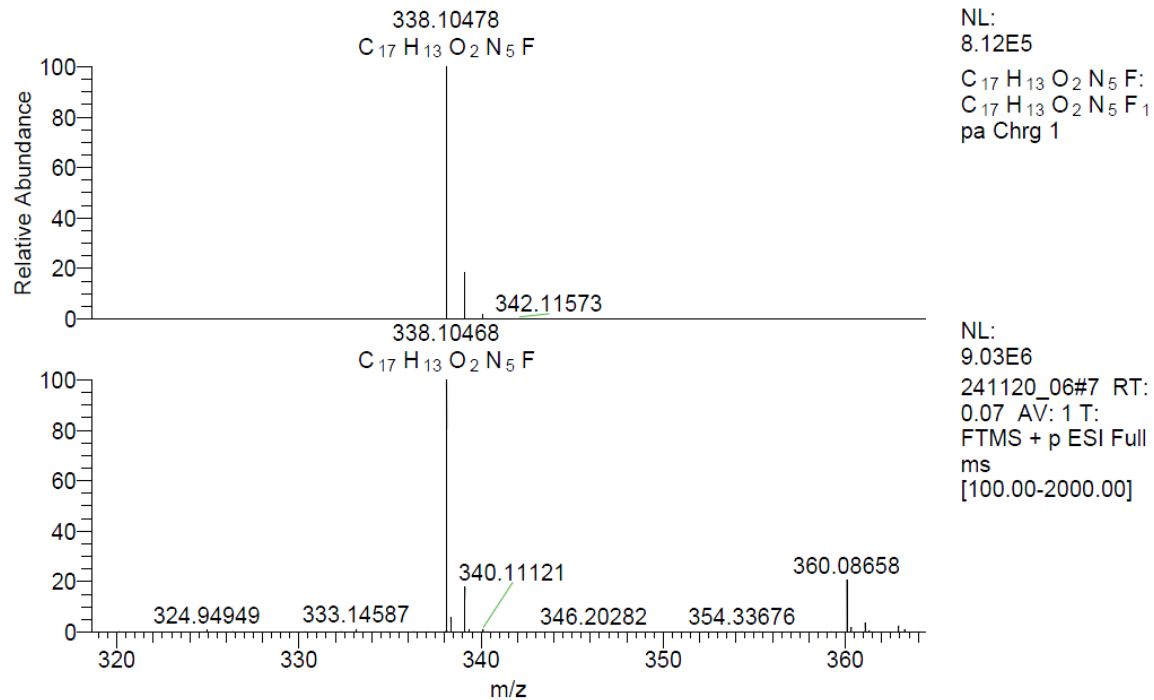
Figure S17. HRMS spectrum of compound 5b
