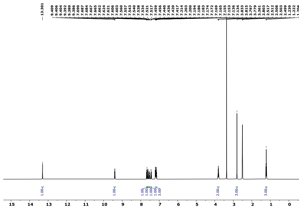
Figure S10. ^1\text{H} NMR (400 MHz, \text{DMSO-}d_6 ) spectrum of compound 8b
