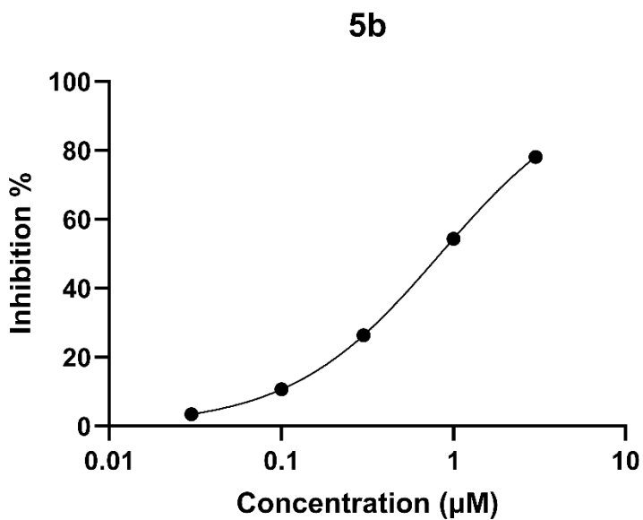
Figure S32. Dose response curve for inhibition % versus concentration ( \mu\text{M} ) of compound 5b
