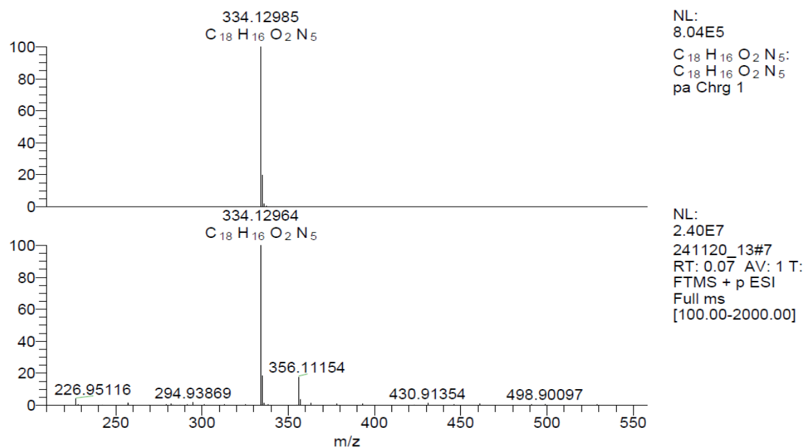
Figure S24. HRMS spectrum of compound 8a
