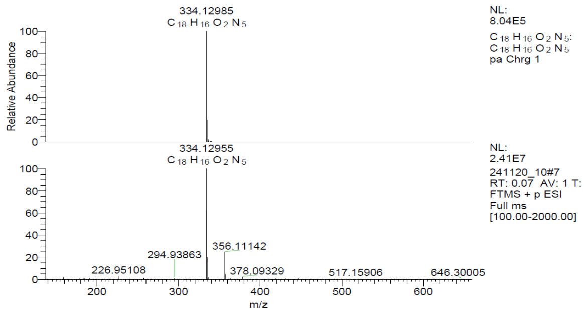
Figure S21. HRMS spectrum of compound 5f
