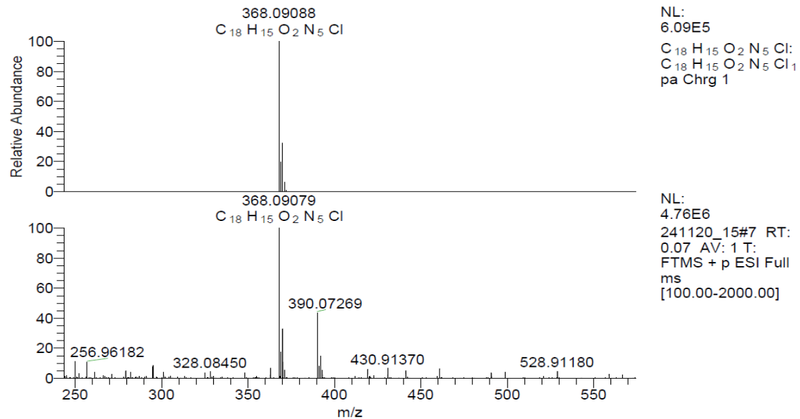
Figure S26. HRMS spectrum of compound 8c
