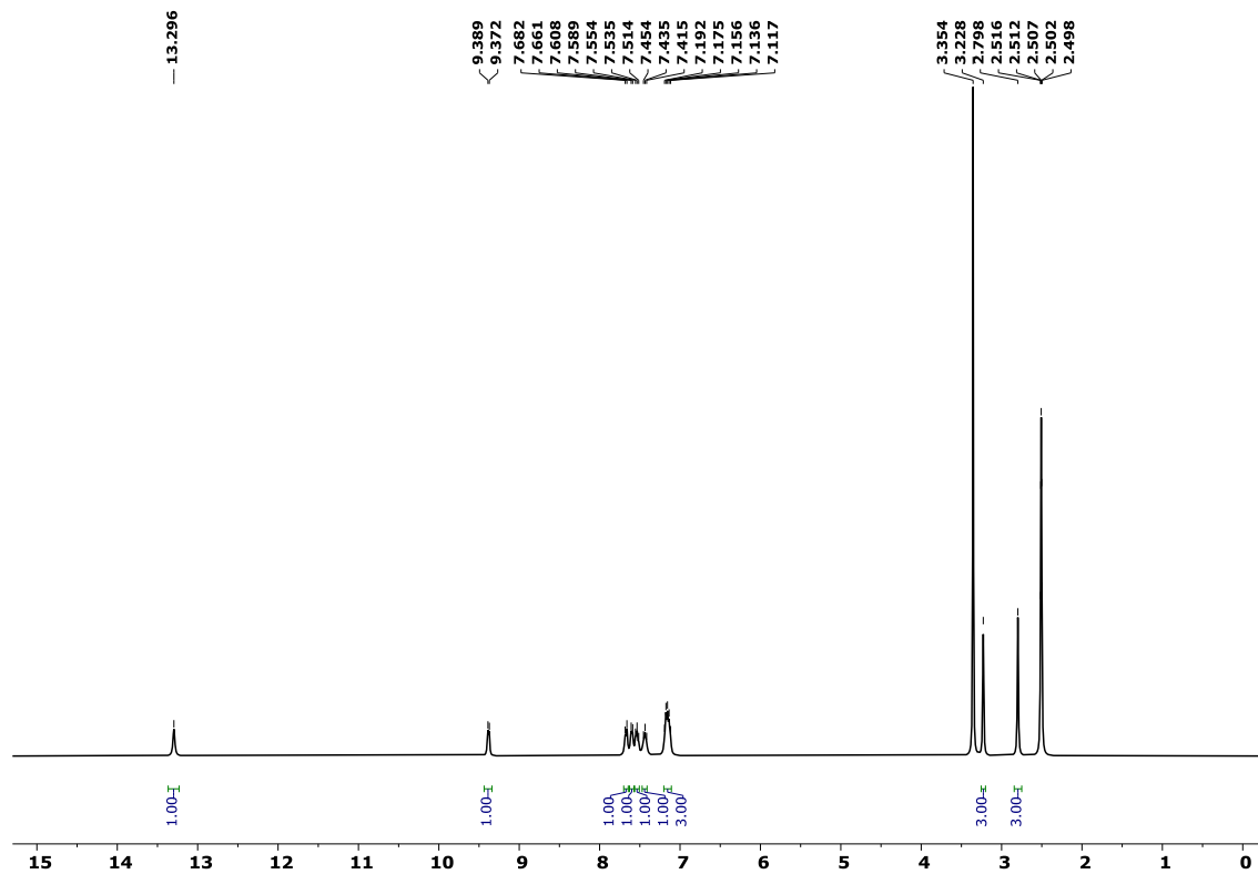
Figure S9. ^1\text{H} NMR (400 MHz, \text{DMSO-}d_6 ) spectrum of compound 8a
