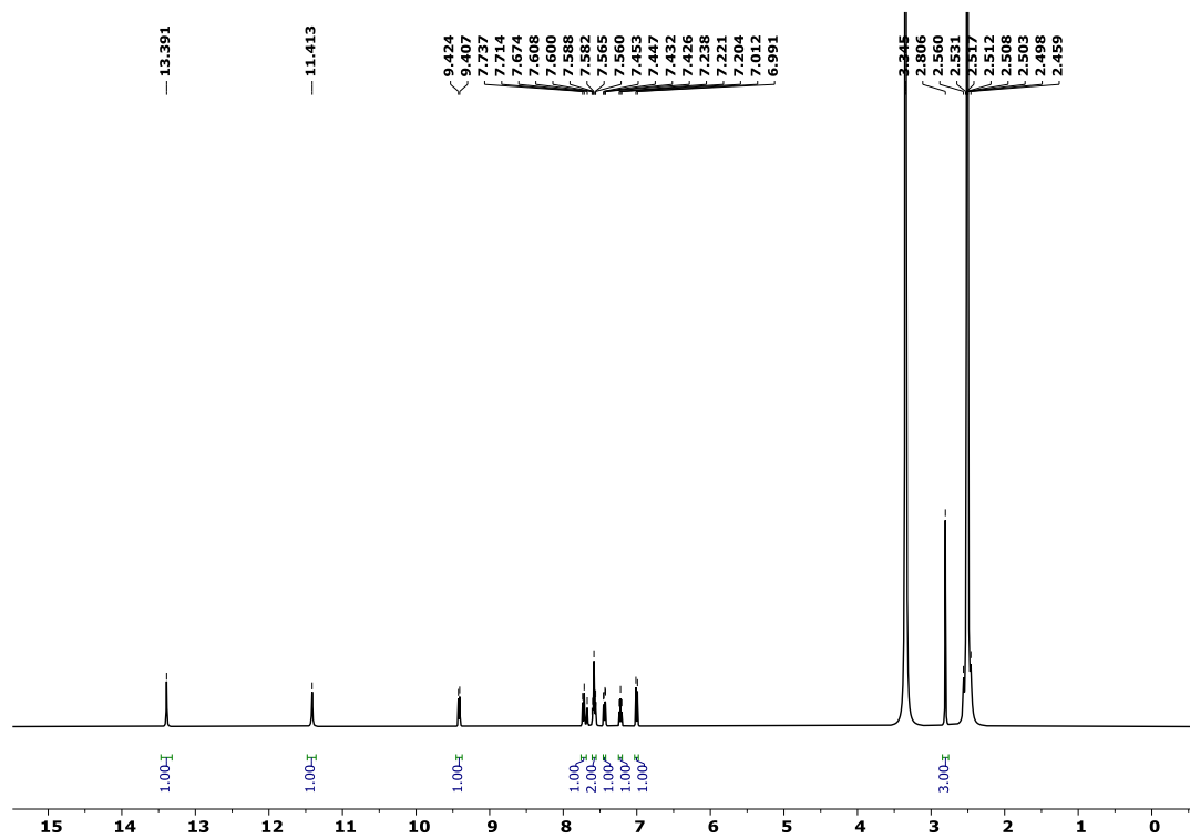
Figure S4. ^1\text{H} NMR (400 MHz, \text{DMSO-}d_6 ) spectrum of compound 5d
