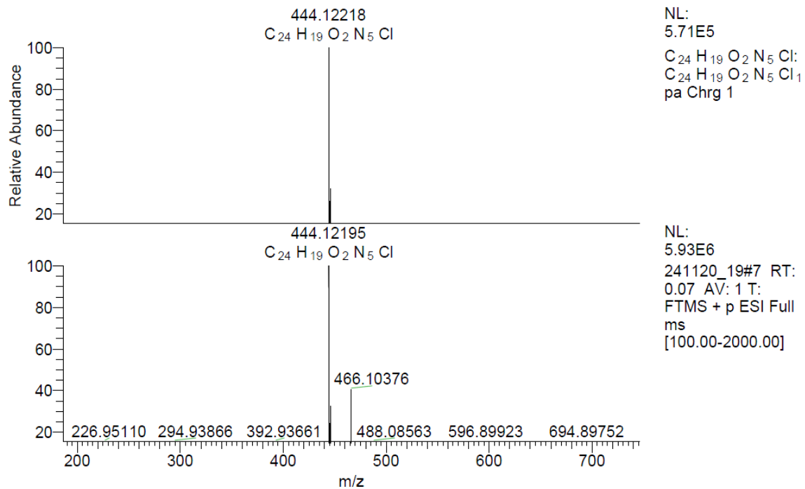
Figure S30. HRMS spectrum of compound 11c
