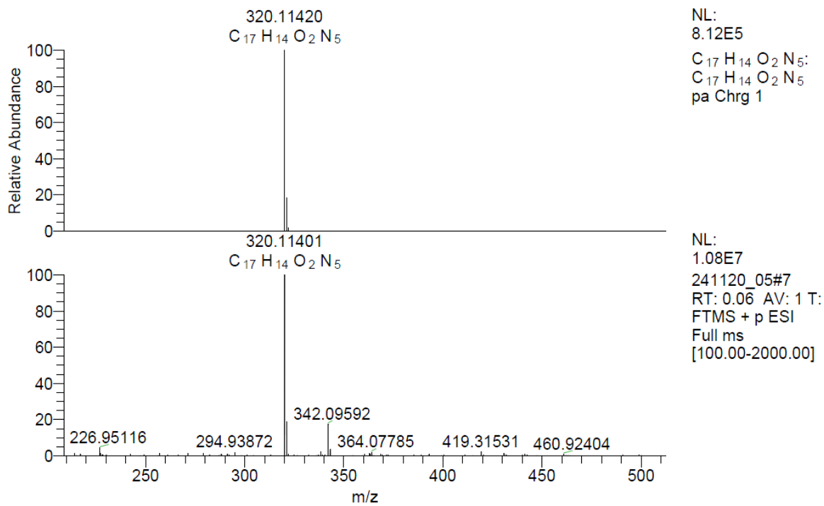
Figure S16. HRMS spectrum of compound 5a
