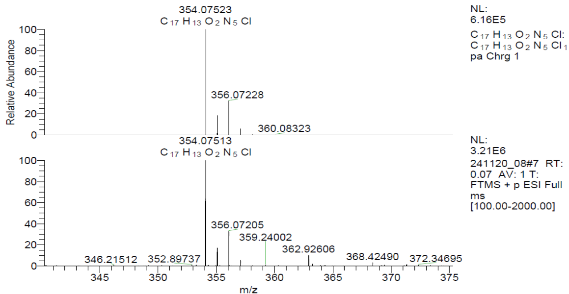
Figure S19. HRMS spectrum of compound 5d
