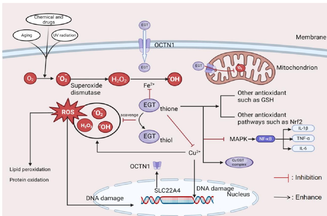
Figure S4. EGT antioxidant and anti-inflammatory mechanism diagram.
